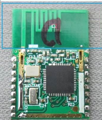
Pcb antenna
