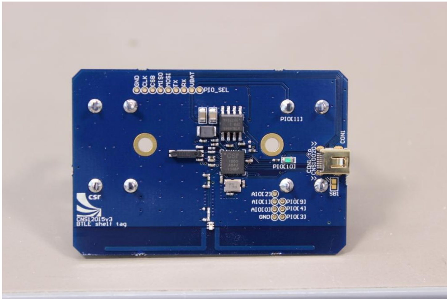
PCB Front
