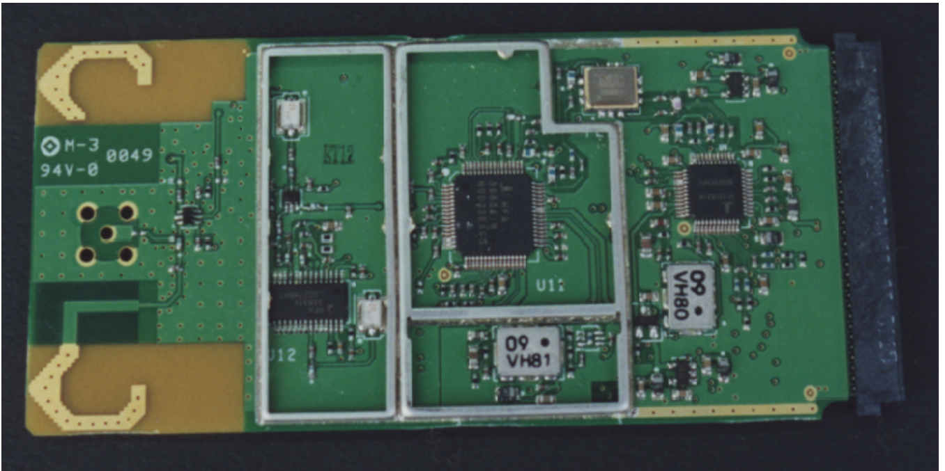
8.4 PBA Bottom View
