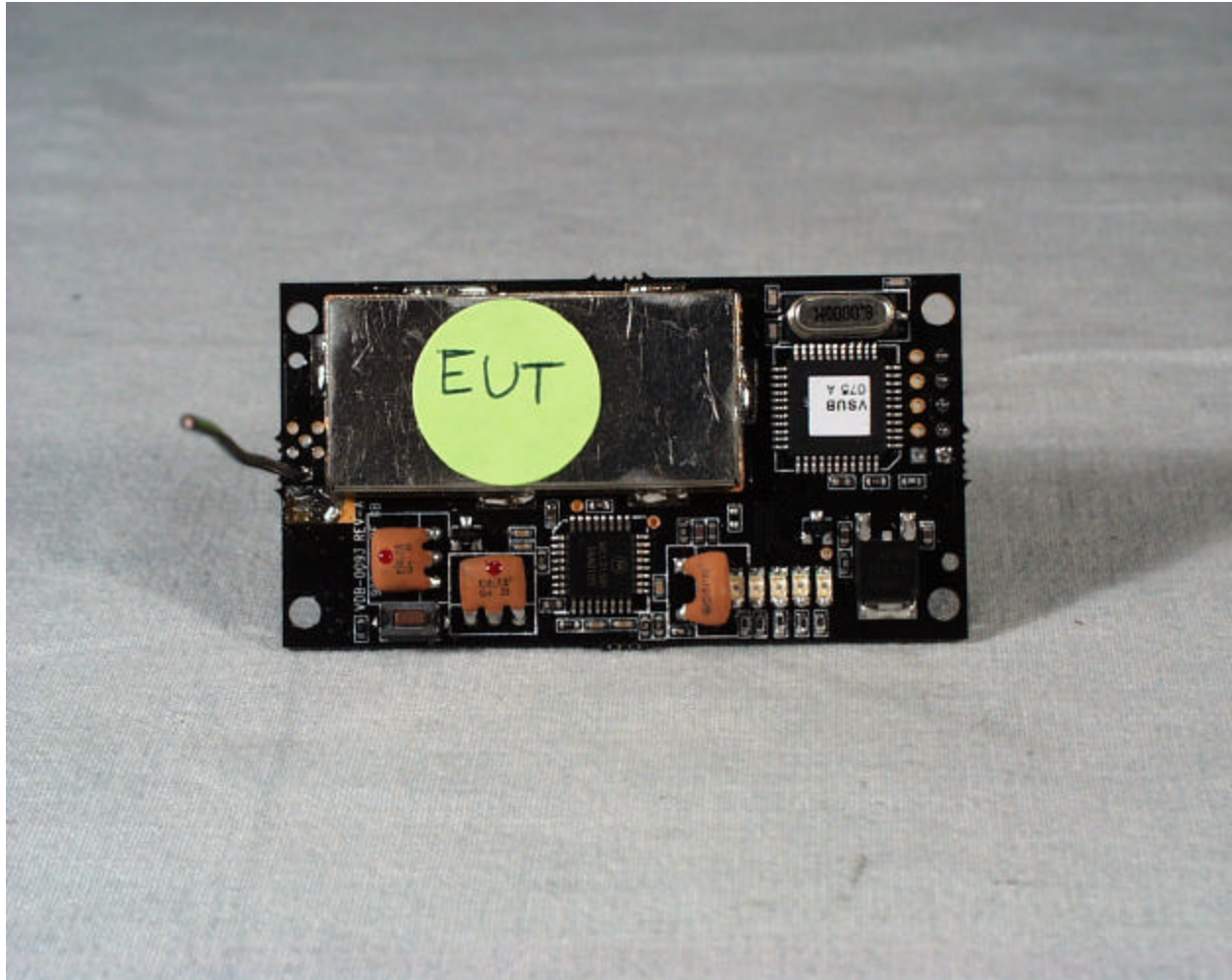
Front View Of The VSUB075(REV A1)
