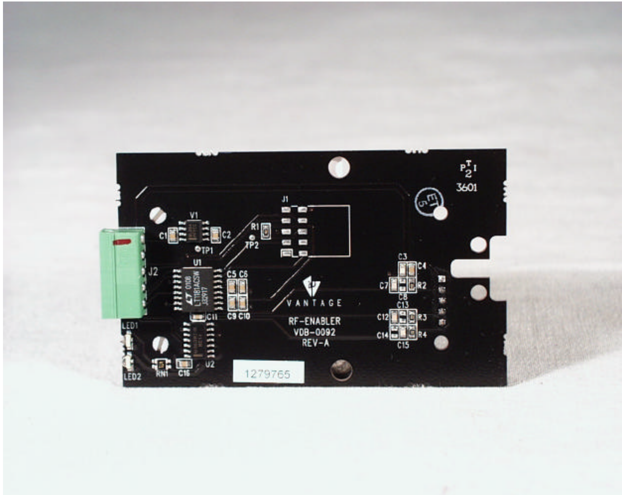
Front View Of The RF Enabler Board
