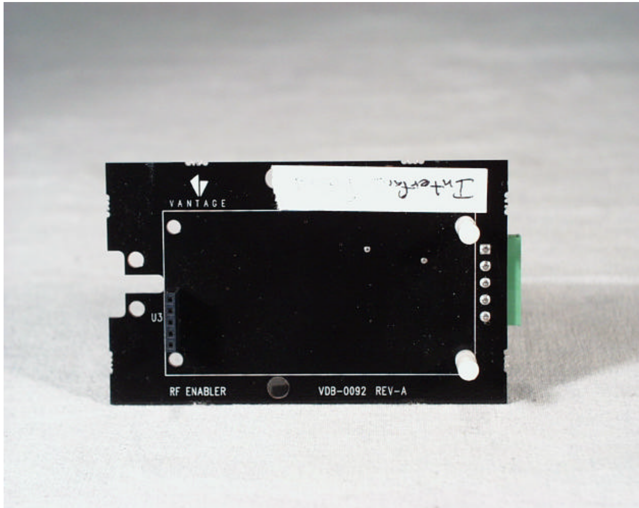
Back View Of The RF Enabler Board
