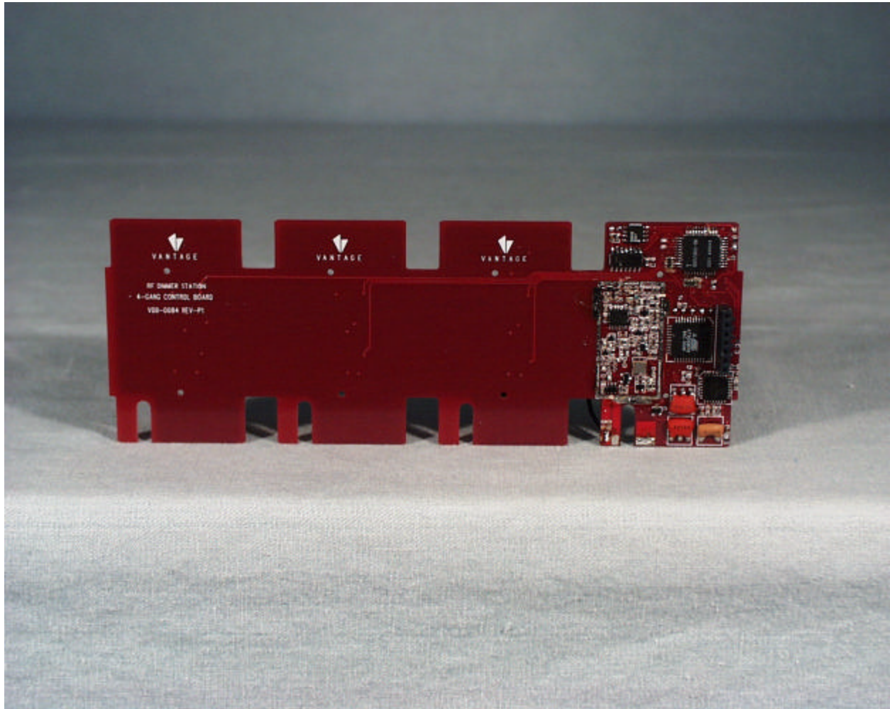
Back View Of The RDS4-2A Control PCB (Shield Removed)
