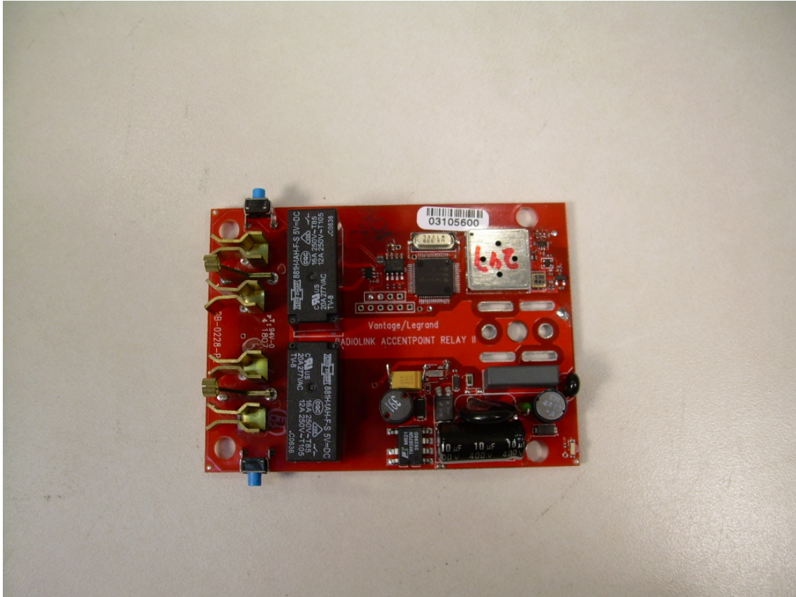
Front Side of the APREL PCB
