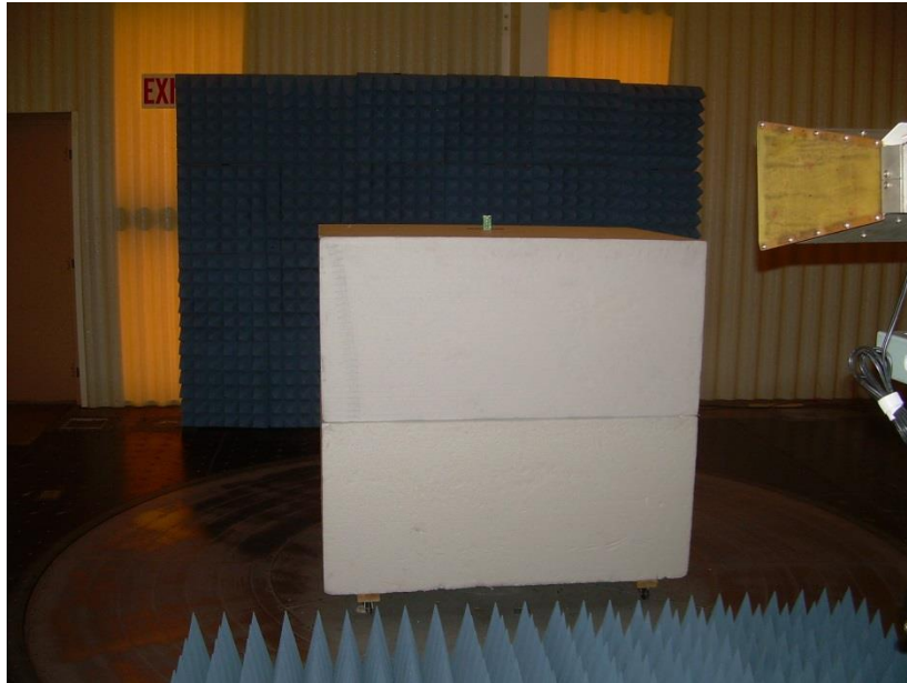
Photograph 3: Front View Radiated Emissions – Above 1000 MHz – Worst-Case Configuration – Vertical Placement
