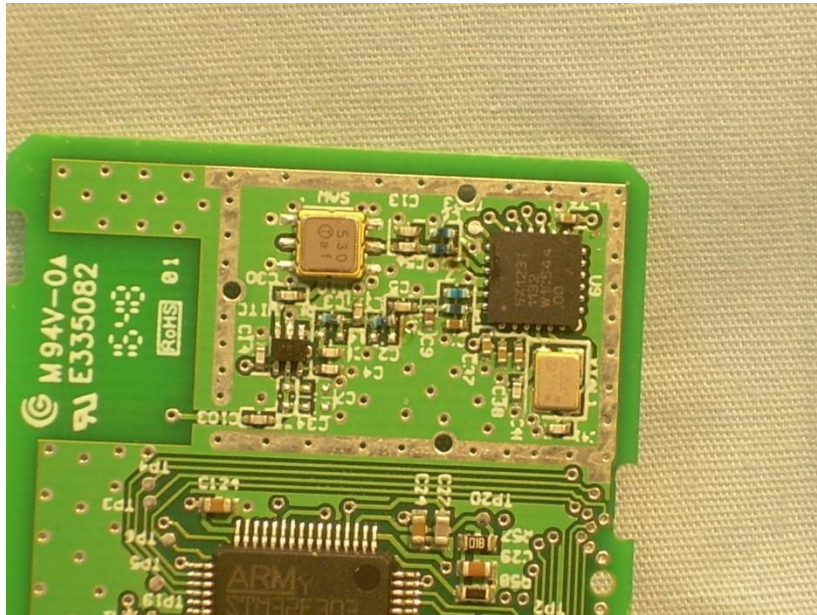
Photograph 12 – Circuitry Under RF Shield
