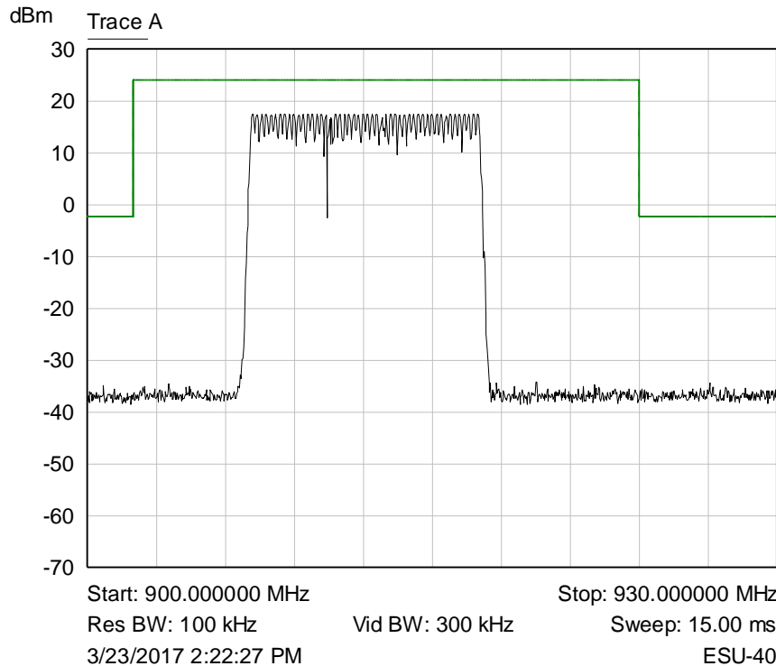
Graph 11: Transmitter Operating Band
