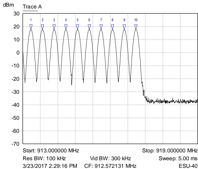
Graph 2: EUT Channel Plot
