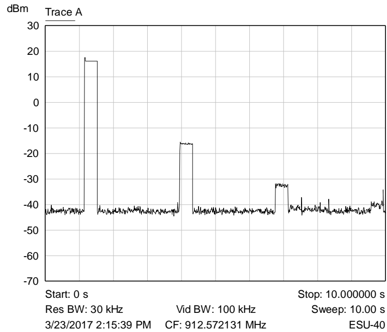
Graph 7: Timing Plot Showing Channel Hits per 10 Seconds
