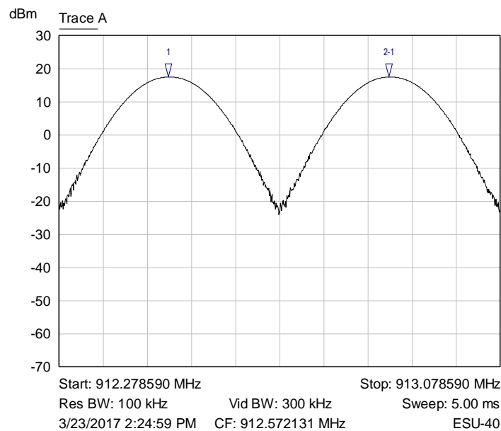
Graph 3: Channel Separation Plot (Modulated Emission)
