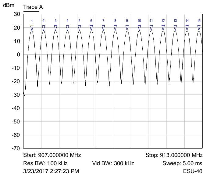
Graph 1: EUT Channel Plot
