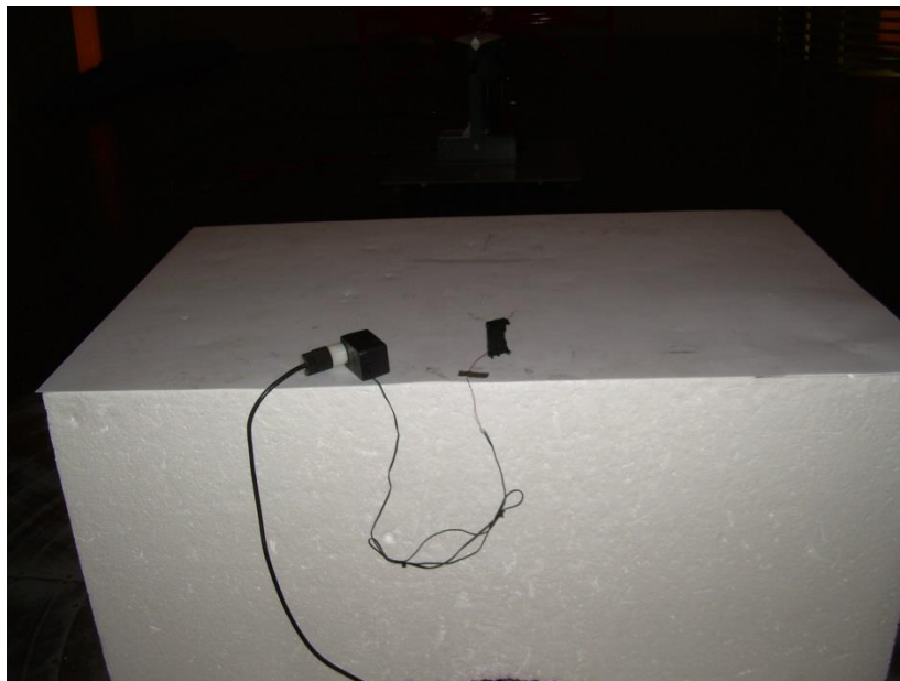
Photograph 2: Back View Radiated Emissions – 30 – 1000 MHz – Worst-Case Configuration – Vertical Placement
