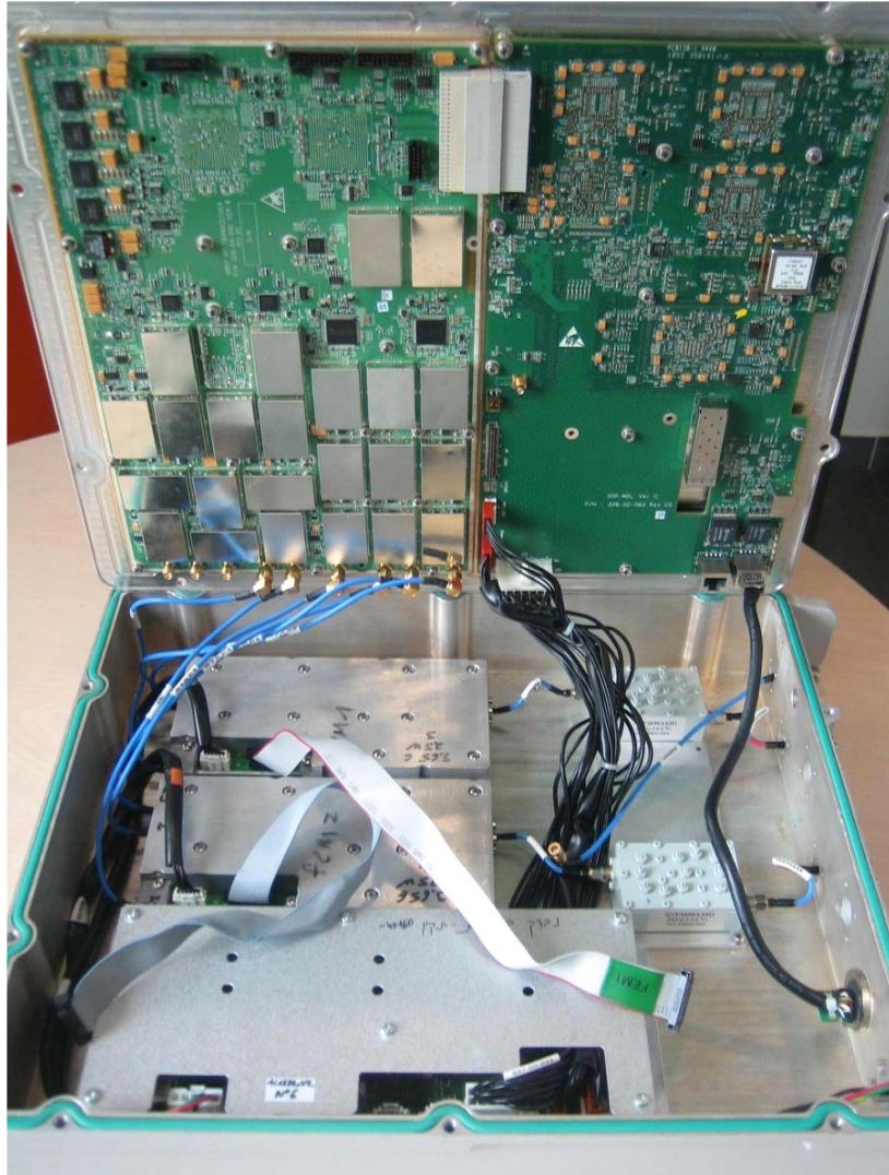
Photograph No.1 "uMAXe/AirGrid 3.65 GHz" internal view
