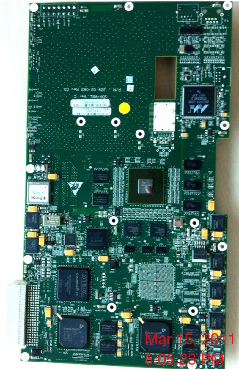
Photograph No.6 "uMAXe/AirGrid 3.65 GHz" digital PCB rear side view
