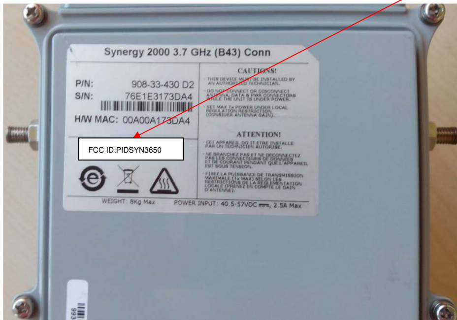
“Synergy 2000, 3.7 GHz” bottom panel, label with FCC ID:PIDSYN3650 location
