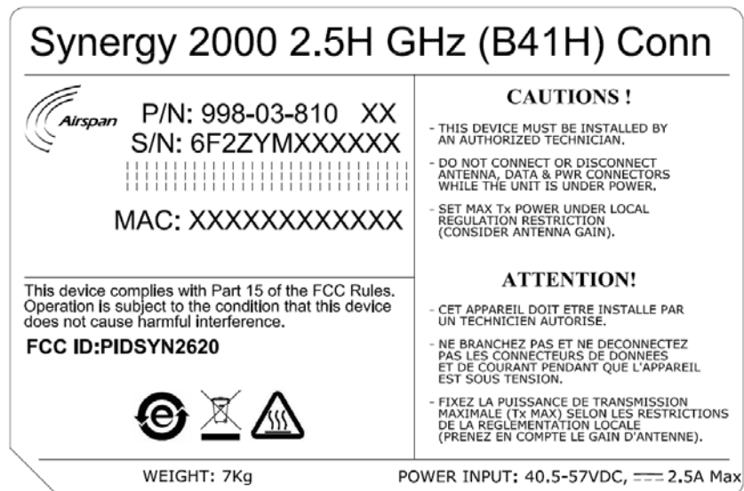
“Synergy 2000 2.5H GHz” bottom panel, label with FCC ID:PIDSYN2620 location
