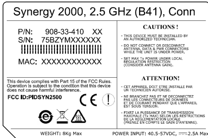
“Synergy 2000 2.5 GHz” bottom panel, label with FCC ID:PIDSYN2500 location
