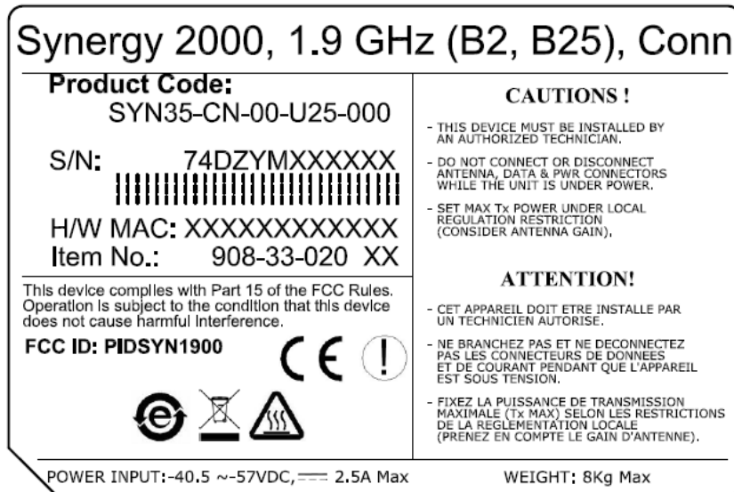
“Synergy 2000, 1.9 GHz” bottom panel, label with FCC ID:PIDSYN1900 location
