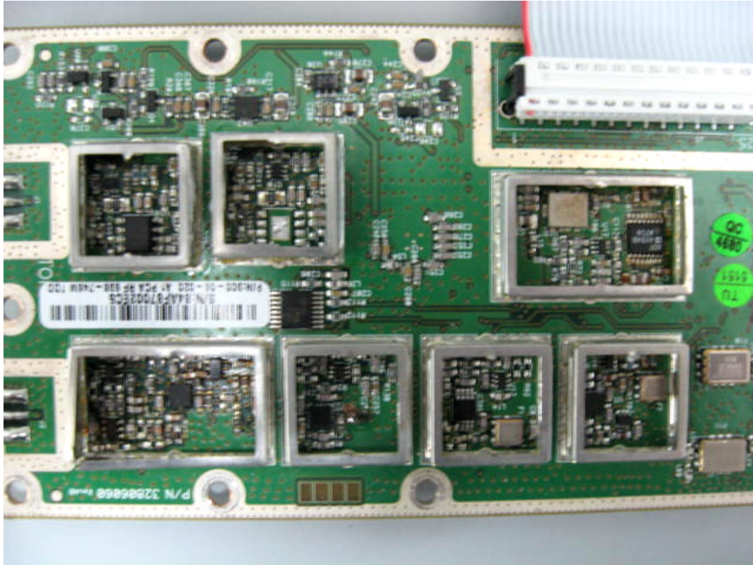
Photograph No5 Close view without shield, PCB left part
