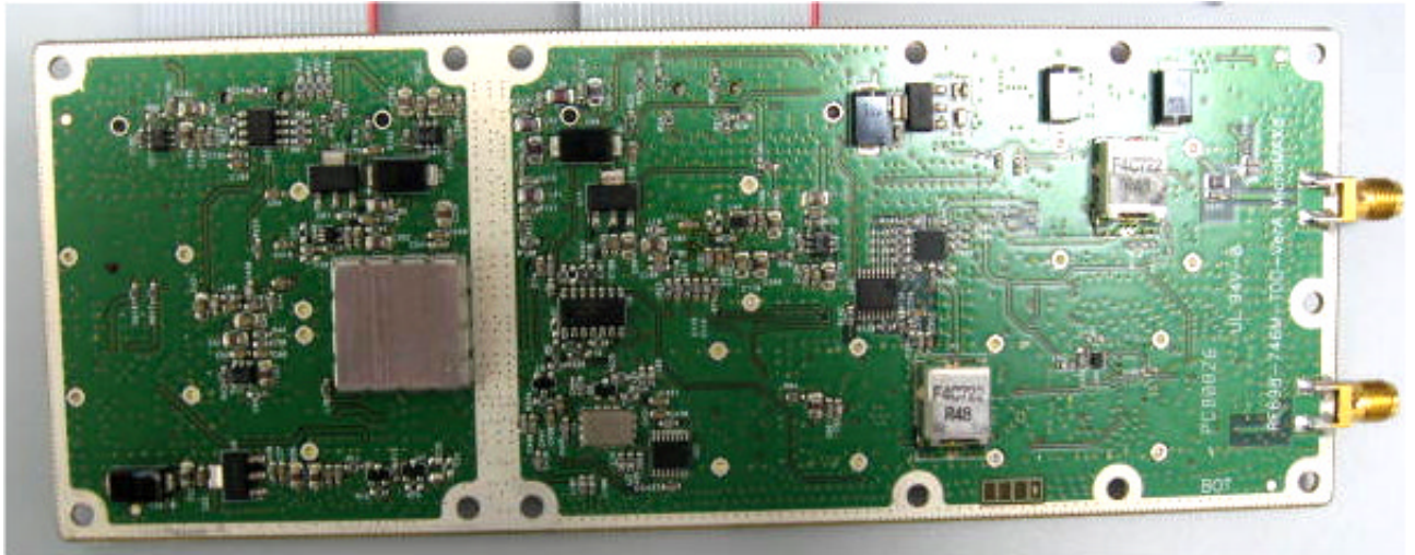
Photograph No8 MicroMAX RF module second side view
