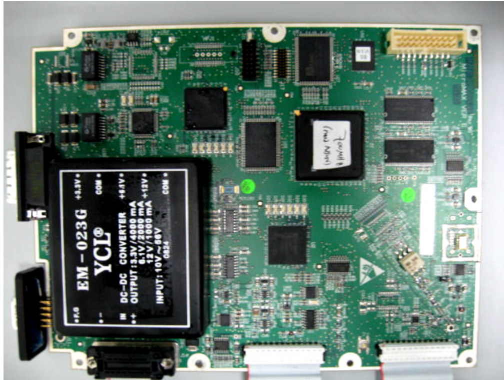
Photograph No.10 Digital interface PCB front view
