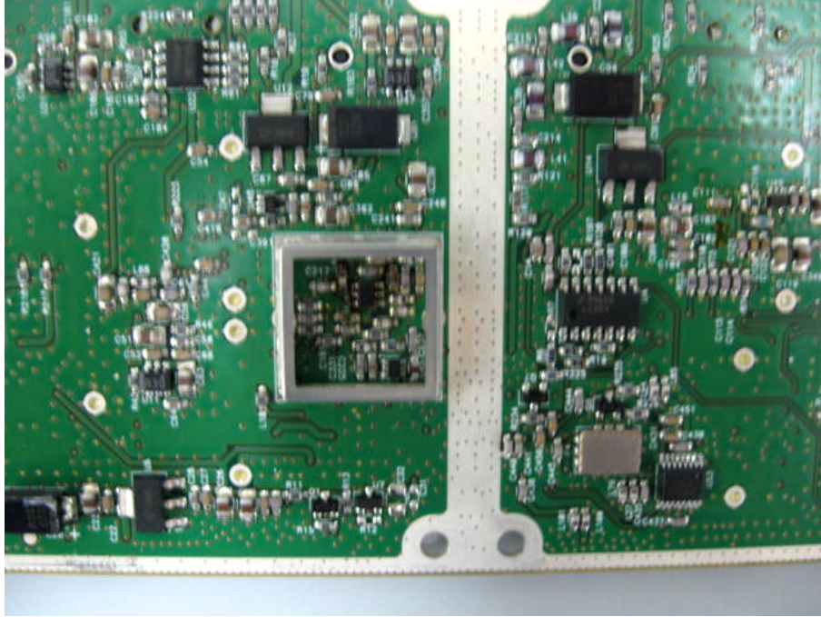
Photograph No9 PCB second side close view without shield
