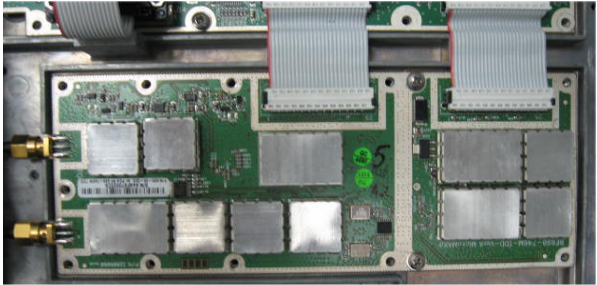
Photograph No3 MicroMAX RF module front view
