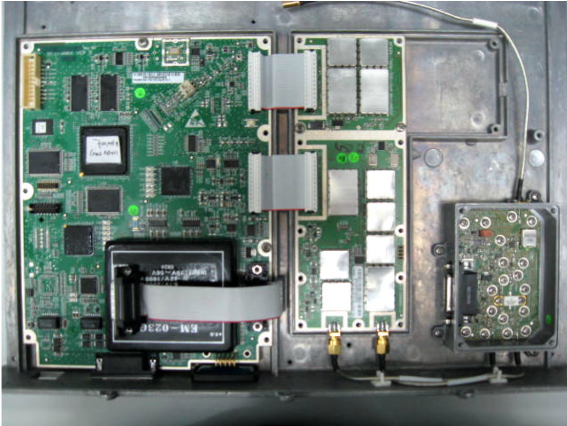
Photograph No2 MicroMAX 698-746M TDD Ext internal view without screens
