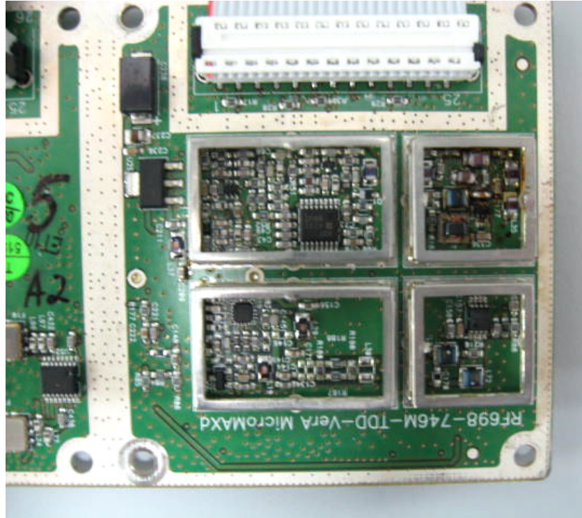
Photograph No7 Close view without shield, PCB right part
