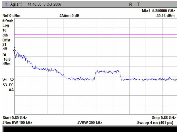
Plot 7.3.21 Spurious emission measurements in 5850 – 5880 MHz range at high carrier frequency
