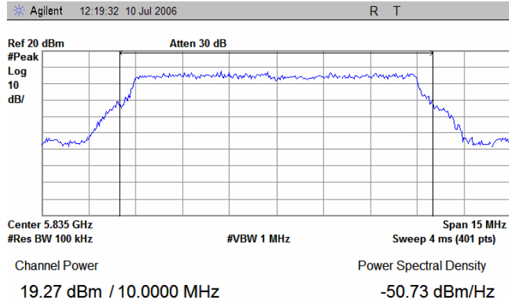
Plot 7.5.9 Peak spectral power density at high frequency within 6 dB band, 10 MHz channel spacing, BPSK
