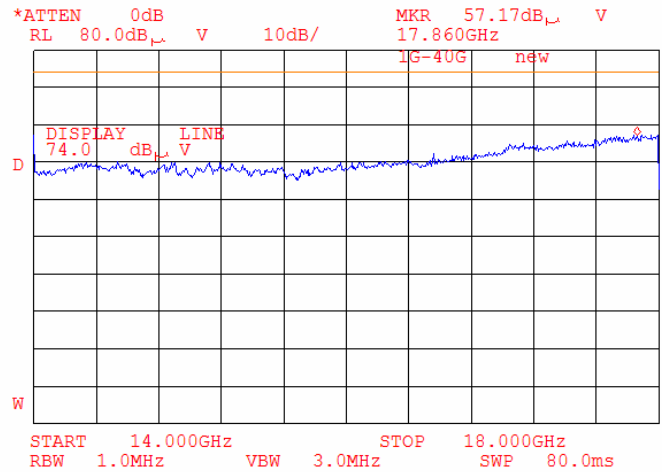
Plot 7.4.36 Radiated emission measurements from 14000 to 18000 MHz at the high carrier frequency
