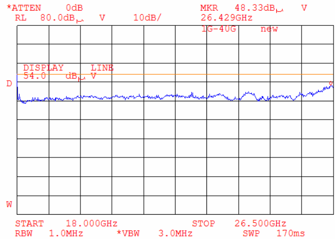
Plot 7.4.38 Radiated emission measurements from 18000 to 26500 MHz at the mid carrier frequency
