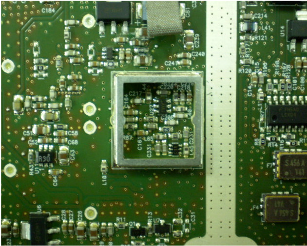
Photograph No.13 PCB second side close view, without shields
