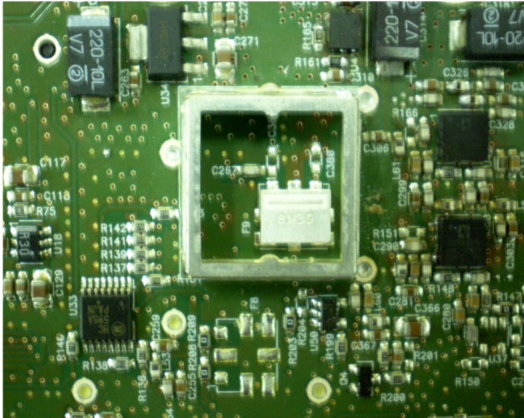
Photograph No.14 PCB second side close view, without shields
