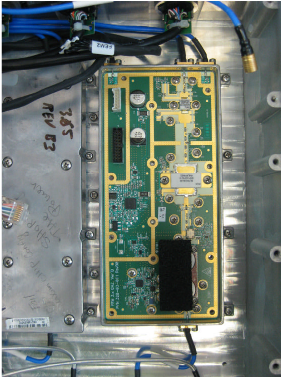
Photograph No.7 RF power amplifier internal view
