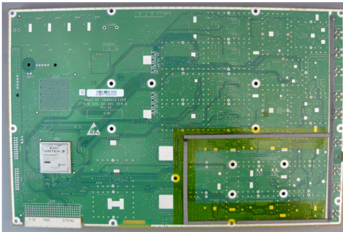
Photograph No.4 "MicroMAXe 3605 3.7 G Ext" RF card second side view
