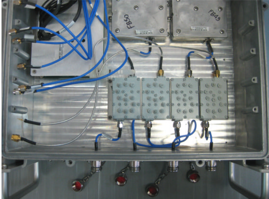
Photograph No.9 "MicroMAXe 3605 3.7 G Ext" RF filters
