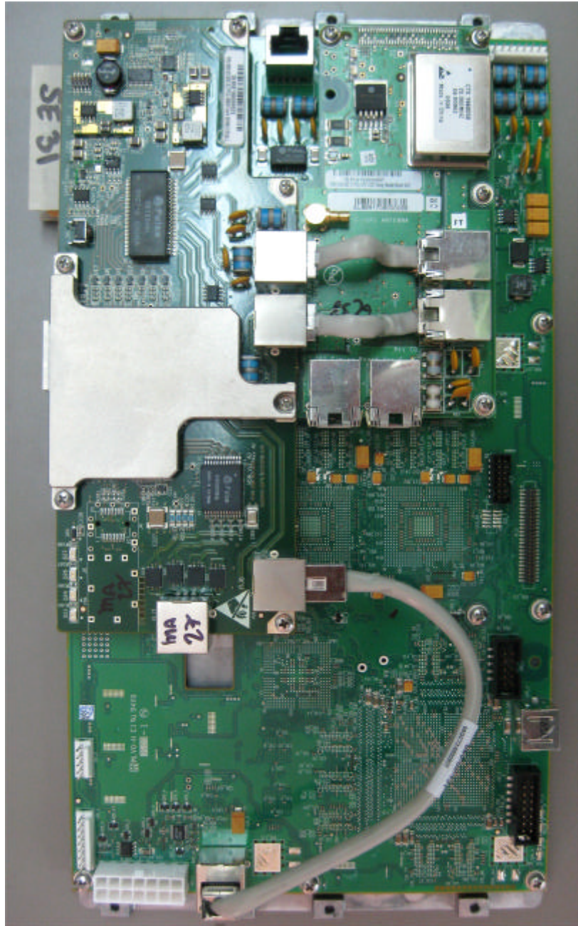
Photograph No.5 Digital PCB front view
