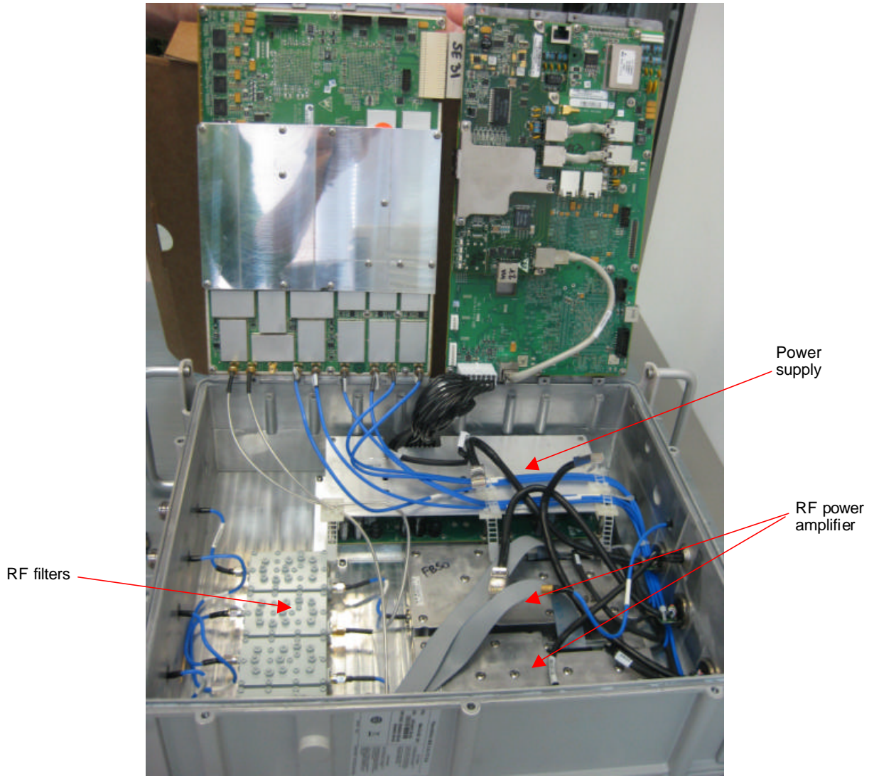
Photograph No.1 "MicroMAXe 3605 3.7 G Ext" internal view
