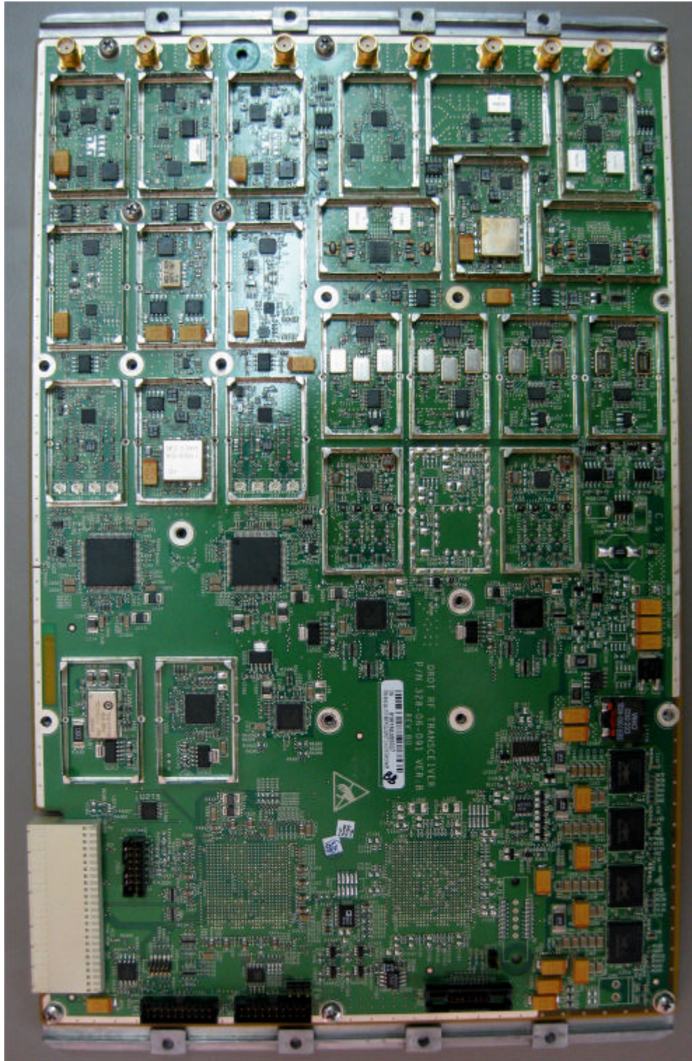
Photograph No.3 "MicroMAXe 3605 3.7 G Ext" RF card without shielding
