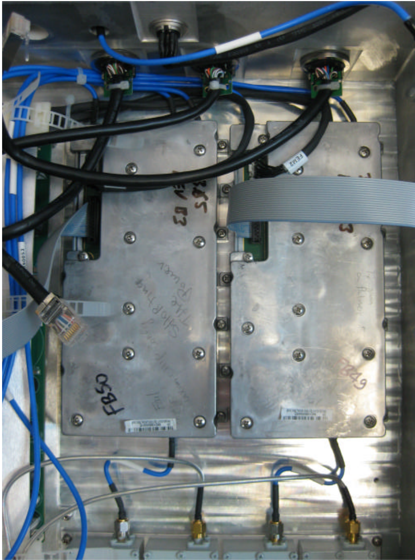
Photograph No.6 "MicroMAXe 3605 3.7 G Ext" RF power amplifiers
