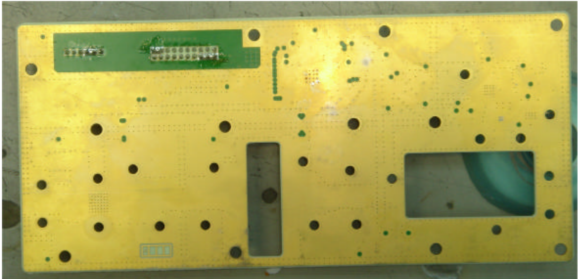
Photograph No.8 Power amplifier PCB second side internal view
