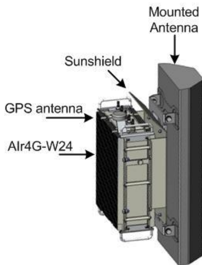
Figure 29 - Antenna mounted on Air4G-W24
