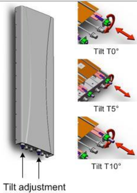
Figure 28 - Variable tilt antenna
