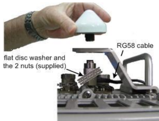
Figure 31 - Attach GPS antenna to RG58 cable
