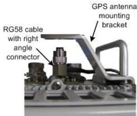
Figure 30 - GPS cable assembly prior to mounting
