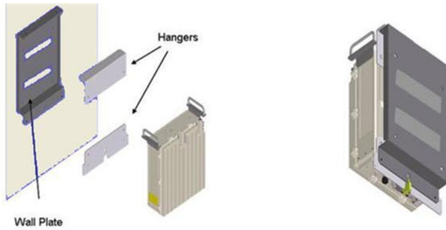
Figure 18 – Wall Mounted Air4G-W24
