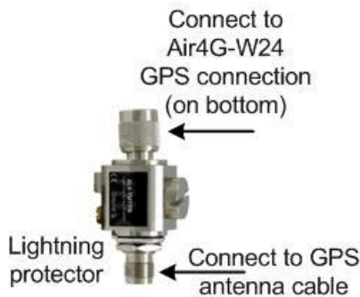
Figure 10 - Lightning/Surge protector (required)
