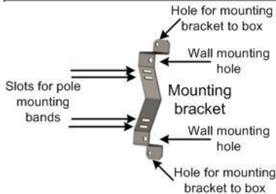
Figure 34 - mounting bracket (2 required)
