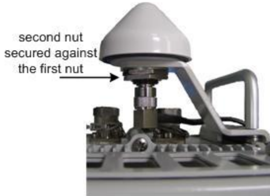
Figure 32 - GPS antenna assembled on bracket
