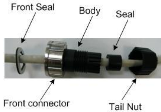
Figure 36 – Ethernet connector cable termination
