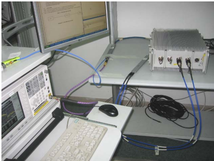
Photograph No.2 Emission mask and conducted spurious emissions measurement setup
