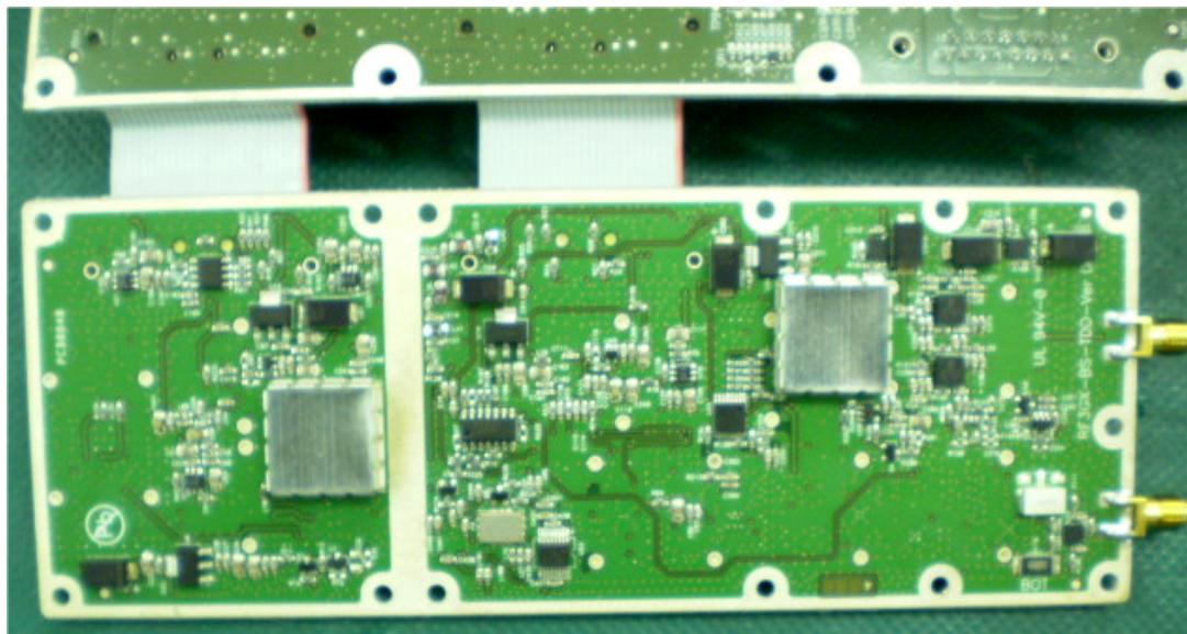
Photograph No.8 MicroMAX RF module second side view
