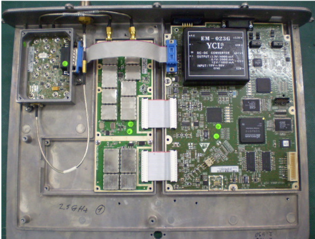
Photograph No.2 MicroMAX 2.5G TDD internal view without screens
