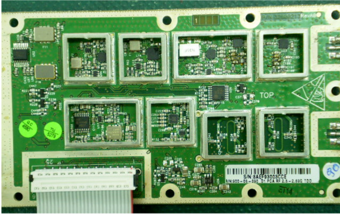
Photograph No.7 Close view without shield, PCB right part
