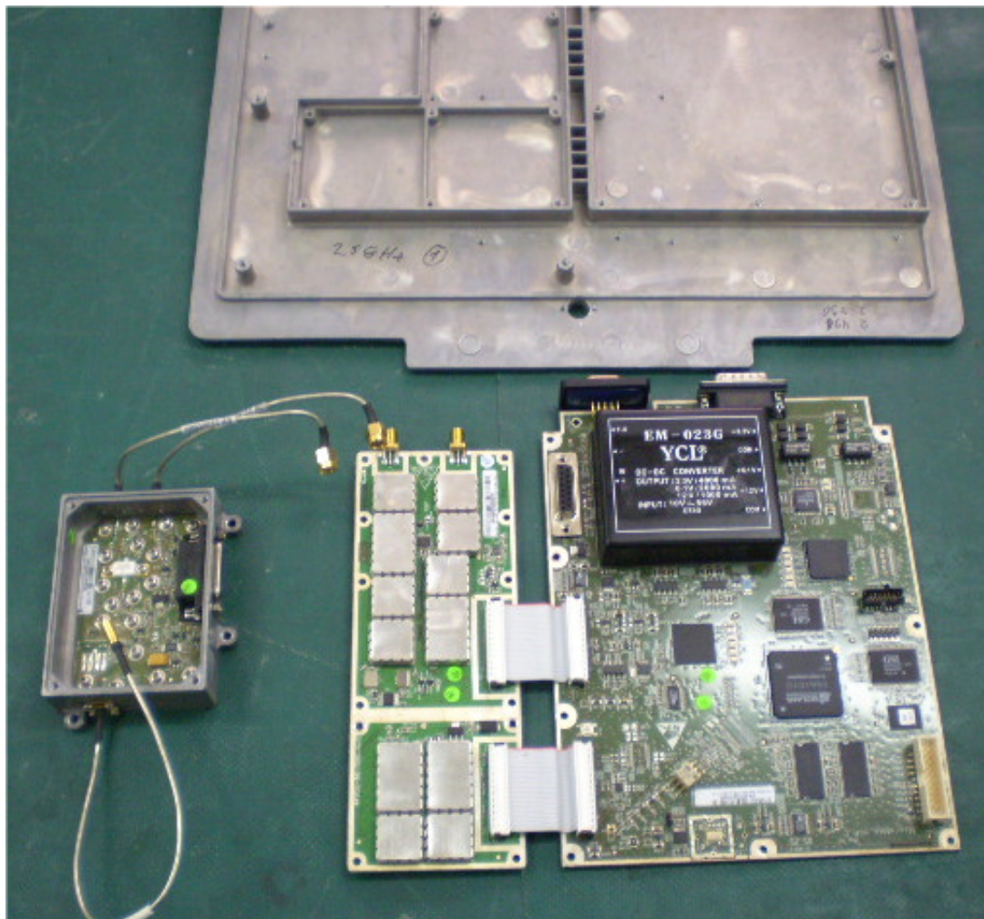
Photograph No.3 MicroMAX 2.5G TDD removed printed circuit boards
