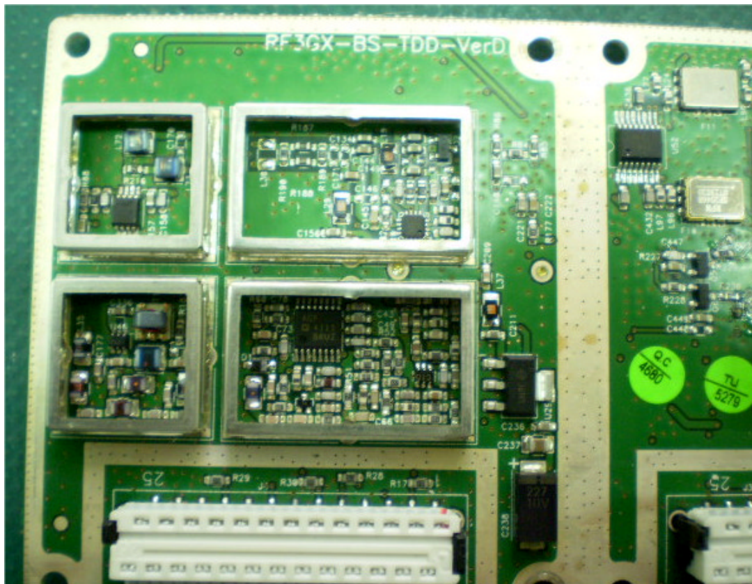
Photograph No.6 Close view without shield, PCB left part
