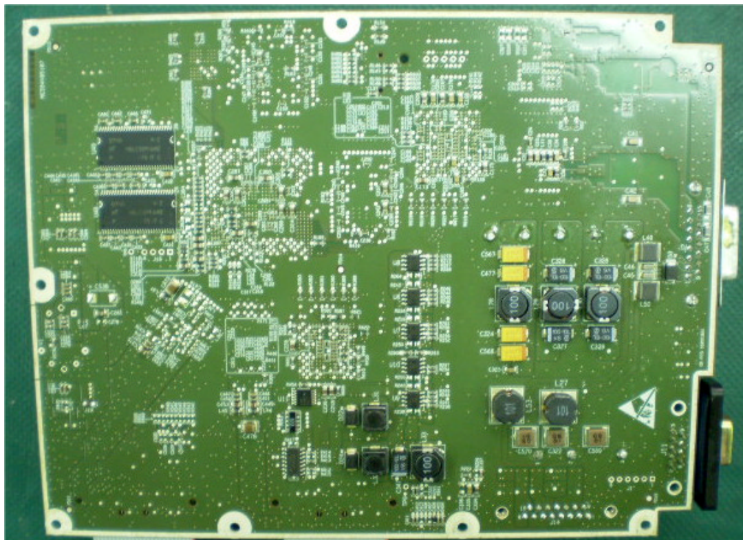
Photograph No.11 Digital interface PCB second side view
