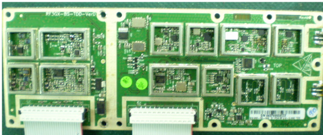
Photograph No.5 RF module without shields
