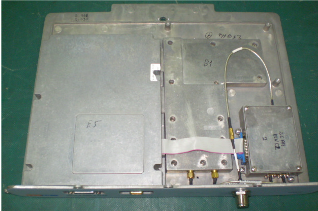
Photograph No.1 MicroMAX 2.5G TDD internal view
