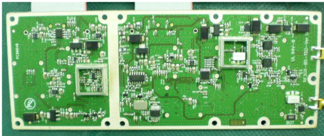
Photograph No.9 PCB second side close view without shield
