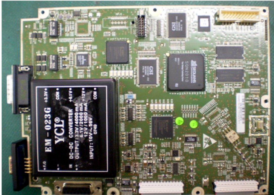
Photograph No.10 Digital interface PCB front view
