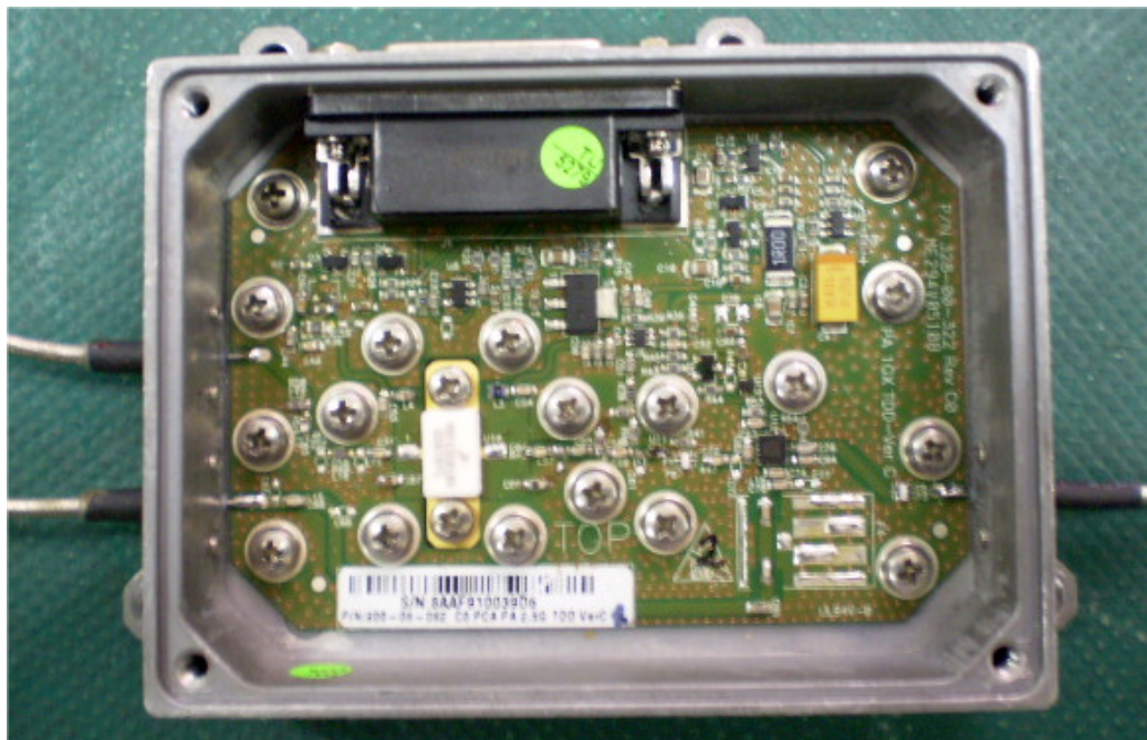
Photograph No.12 Power amplifier (PA) internal view
