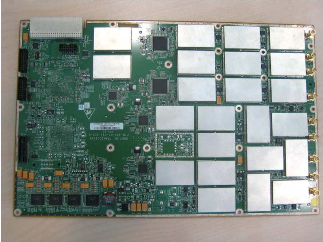
Photograph No.2 “Air4G-MacroMAXe 2310L” RF card front view
