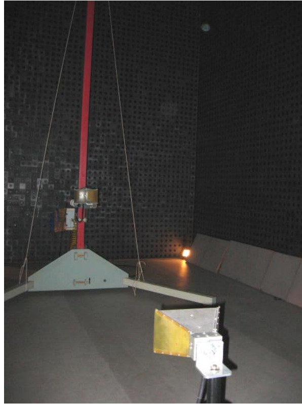
Photograph No.6 Setup of substitution ERP measurements of spurious in the anechoic chamber
