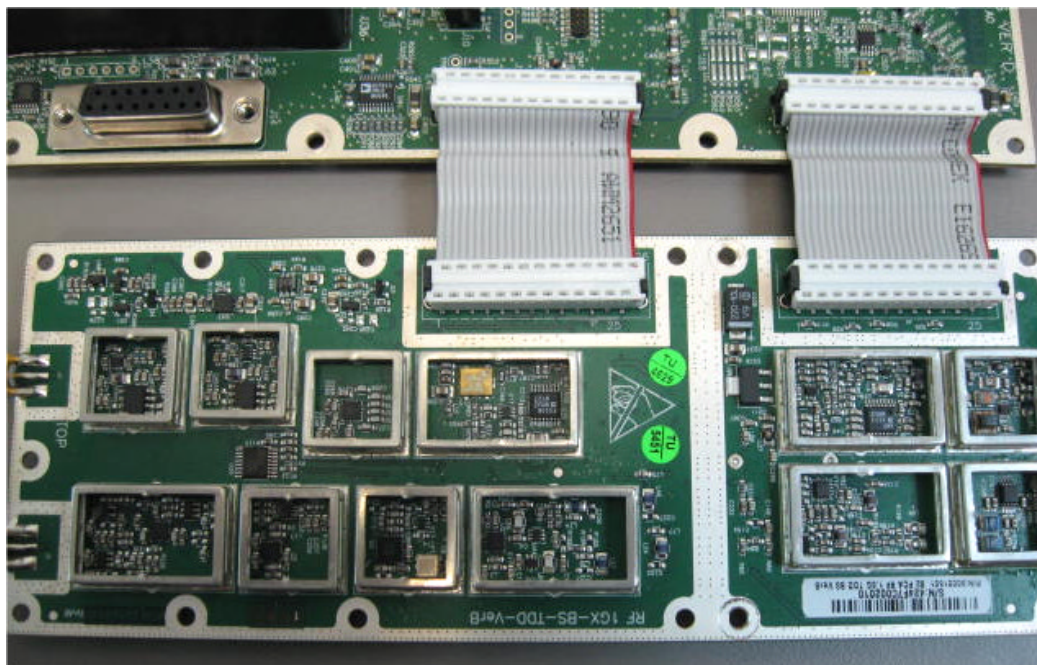
Photograph No.6 RF module without shields
