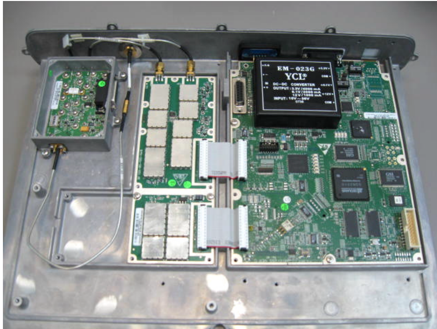
Photograph No.2 MicroMAX 1.4G TDD internal view without screens
