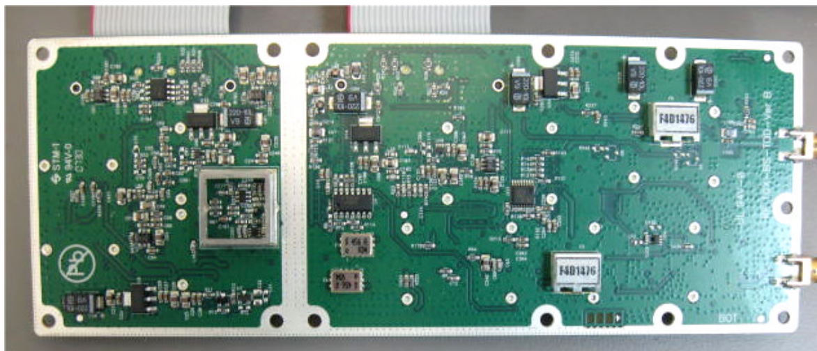
Photograph No.10 PCB second side close view without shield
