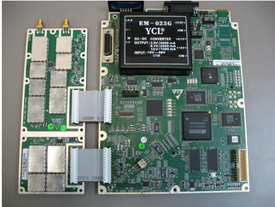
Photograph No.3 MicroMAX 1.4G TDD printed circuit boards front view
