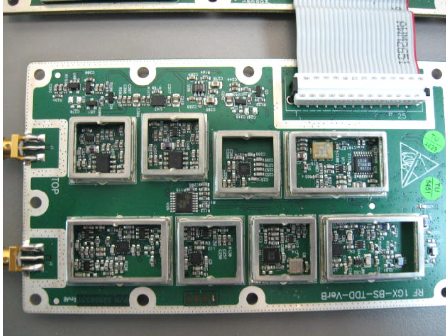
Photograph No.7 Close view without shield, PCB left part
