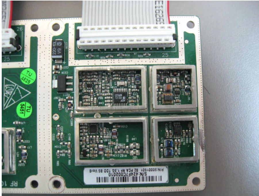
Photograph No.8 Close view without shield, PCB right part
