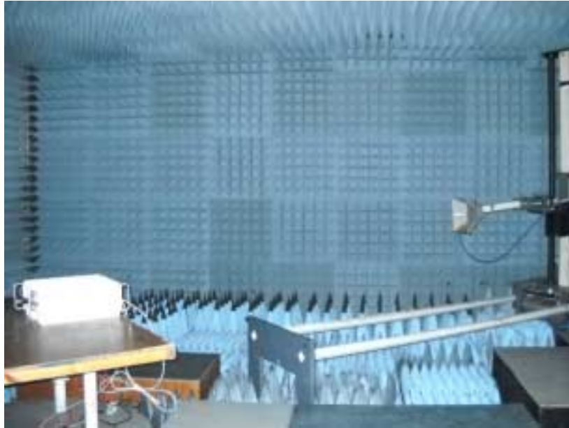
Photograph No.6 Radiated emissions measurement setup in the anechoic chamber above 1000 MHz
