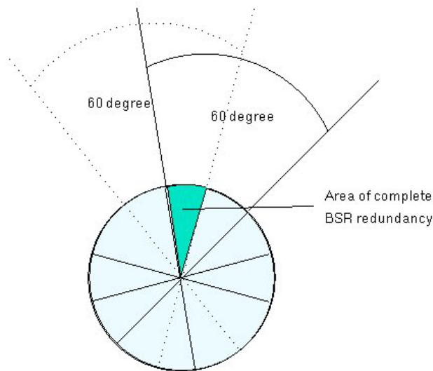
Figure 1-8: Base Station Sector
