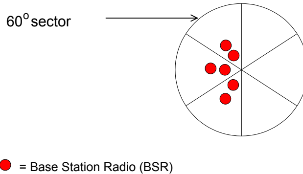
Figure 1-7: Base Station with Complete BSR Redundancy
