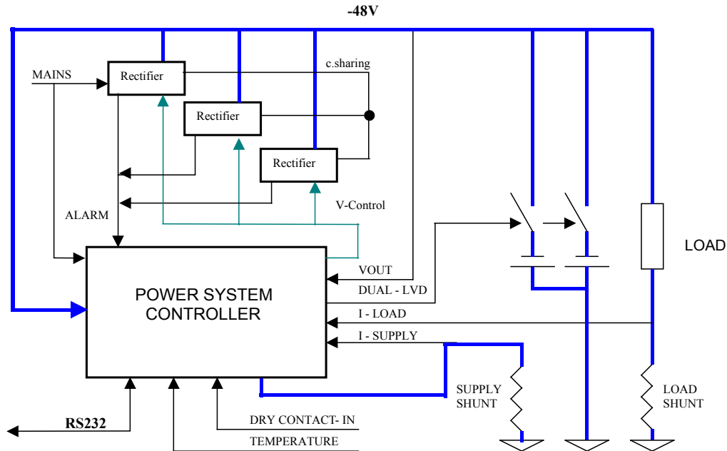
Figure 8-1: BSPS Block Diagram
