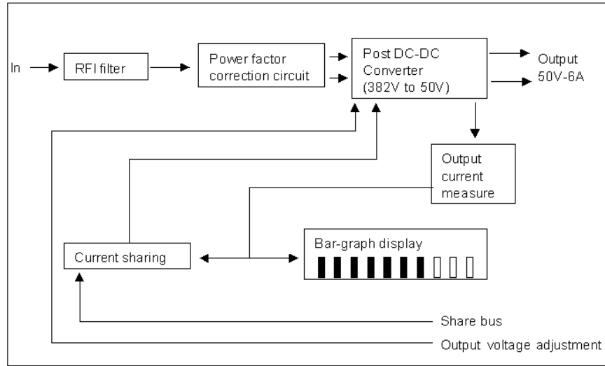
Figure 8-8: BPS Rectifier - Simplified Block Diagram
