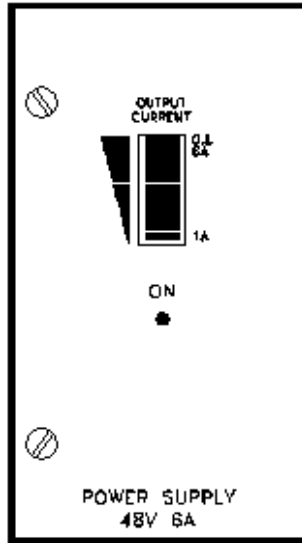
Figure 8-9: BSPS Rectifier Module - Front Panel
