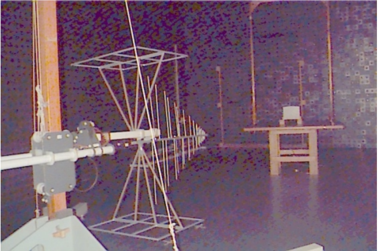
Photograph No.3 Radiated emission measurement test setup
