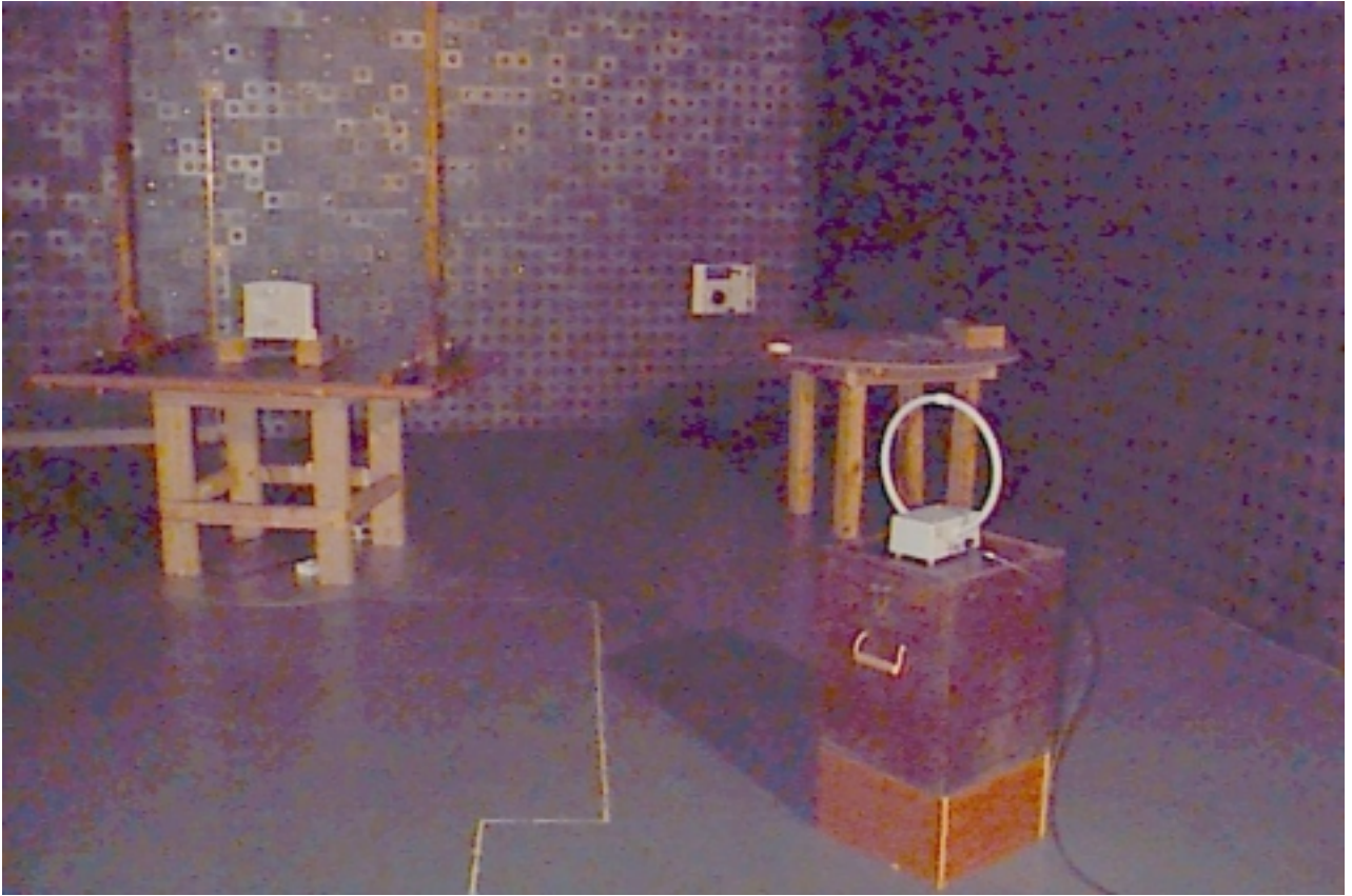
Photograph No.4 Radiated emission measurement test setup
