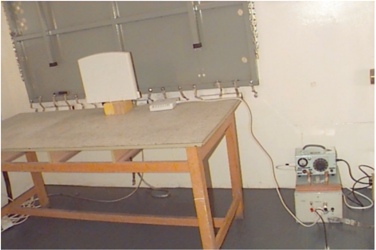
Photograph No.5 Conducted emission measurement test setup
