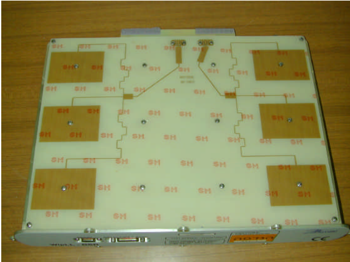
FCC ID:PIDMARCONI; BSR-2.4 inside view (antenna)
