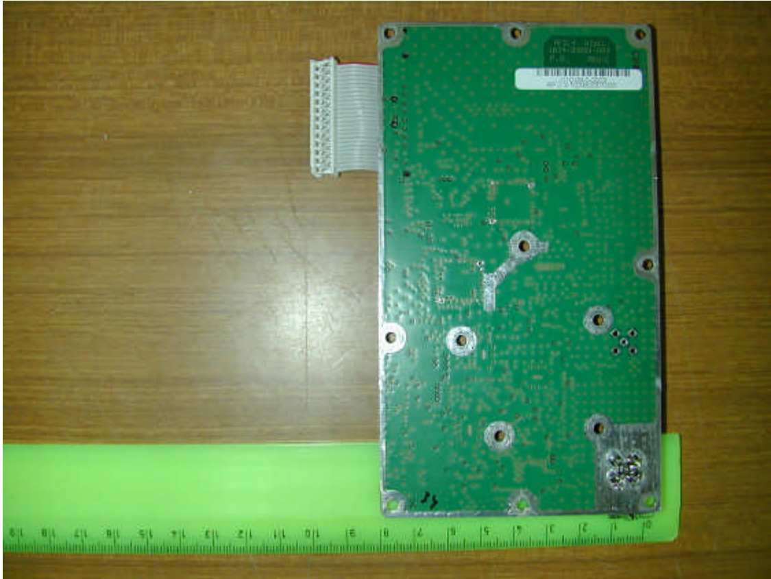
FCC ID:PIDMARCONI; BSR-RF2.4 board, printed side
