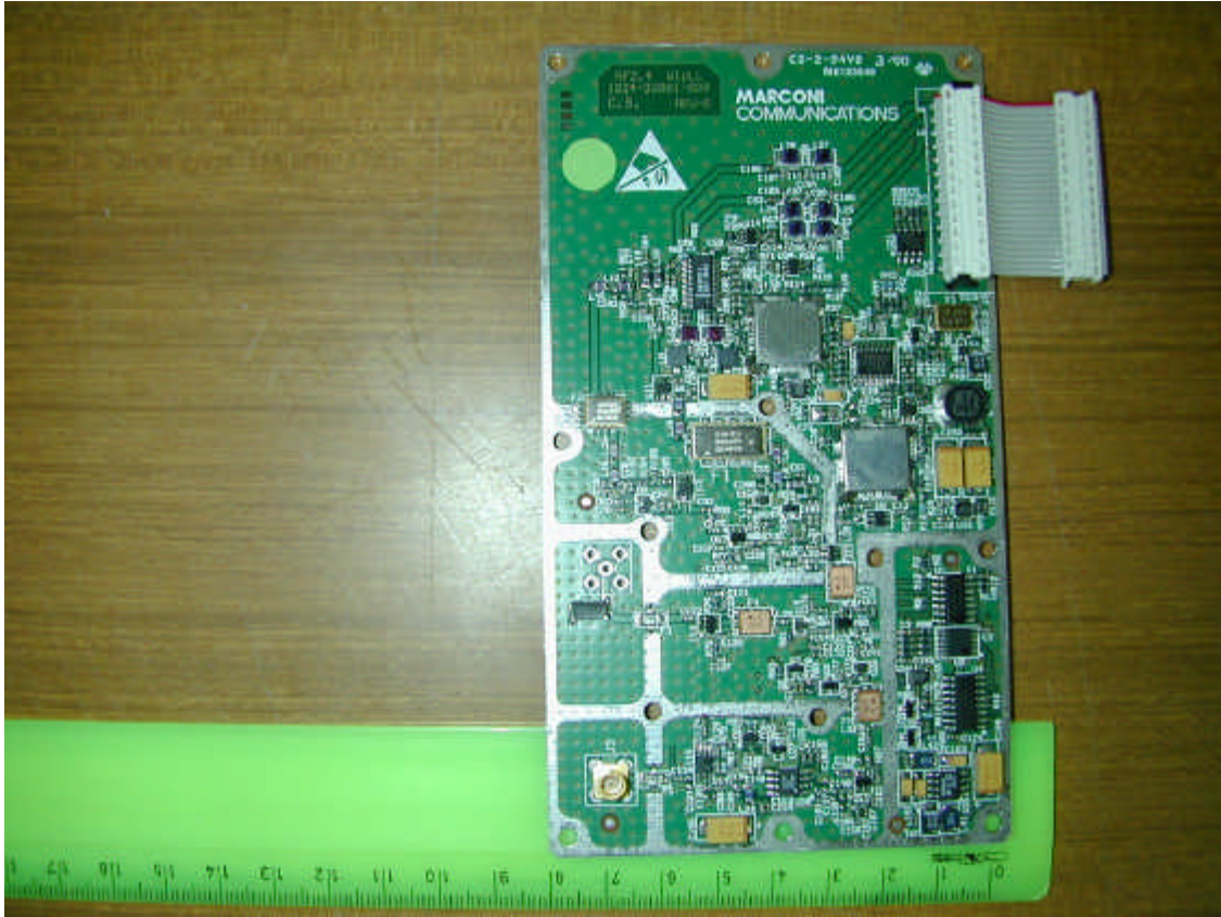
FCC ID:PIDMARCONI; BSR-RF2.4 board, component side
