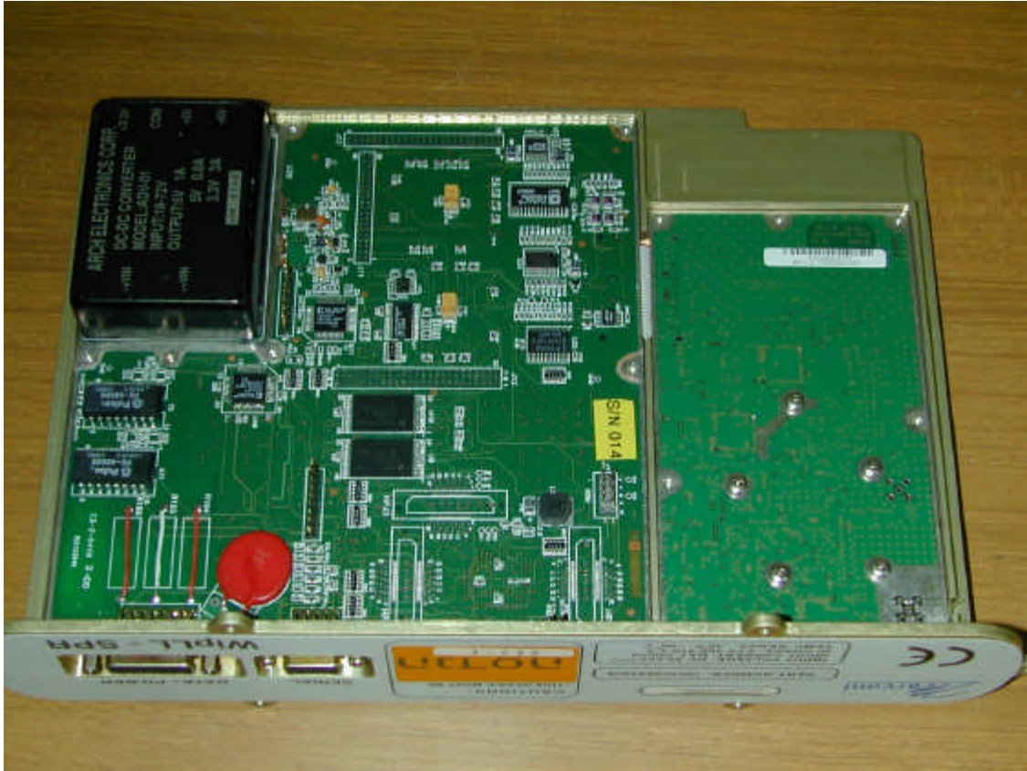
FCC ID:PIDMARCONI; SPR-2.4 inside view without covers
