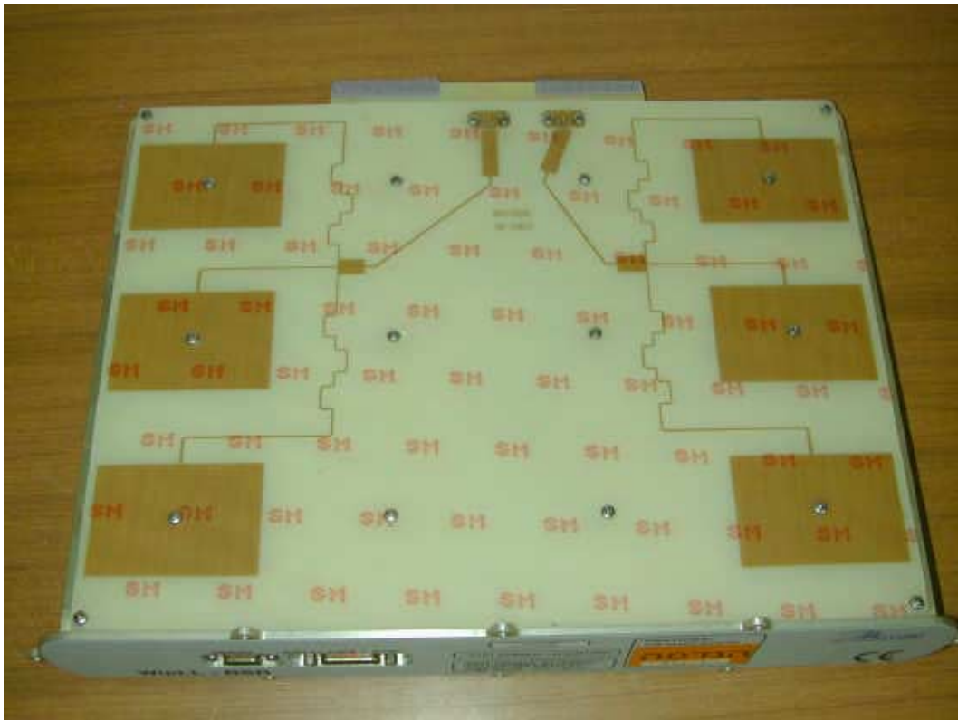
FCC ID:PIDMARCONI; BSR-2.4 inside view (antenna)
