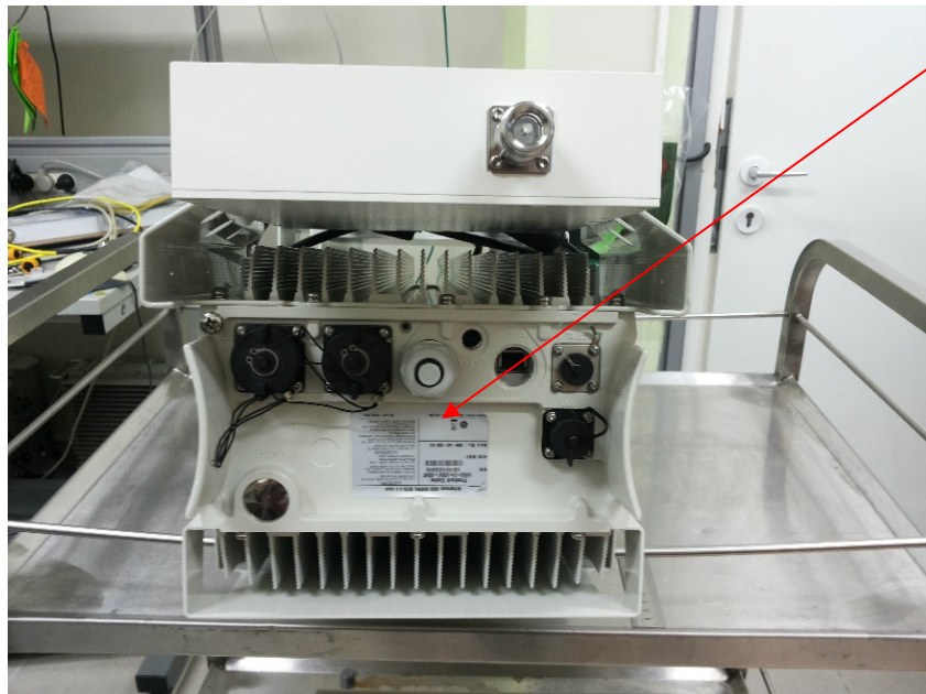
“AirHarmony 4000 866 MHz (B26)”bottom panel, label with FCC ID:PIDHAR4K85 location
