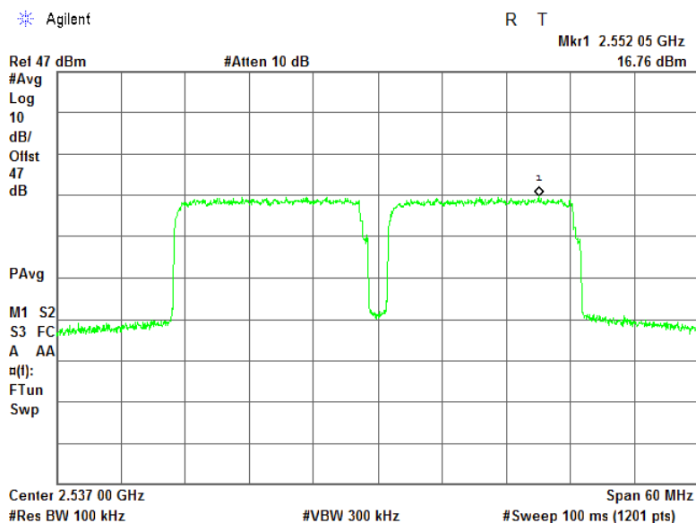
Plot 7.2.11 Power spectral density test results at mid frequency, 64QAM, 40 MHz EBW RF # 2
