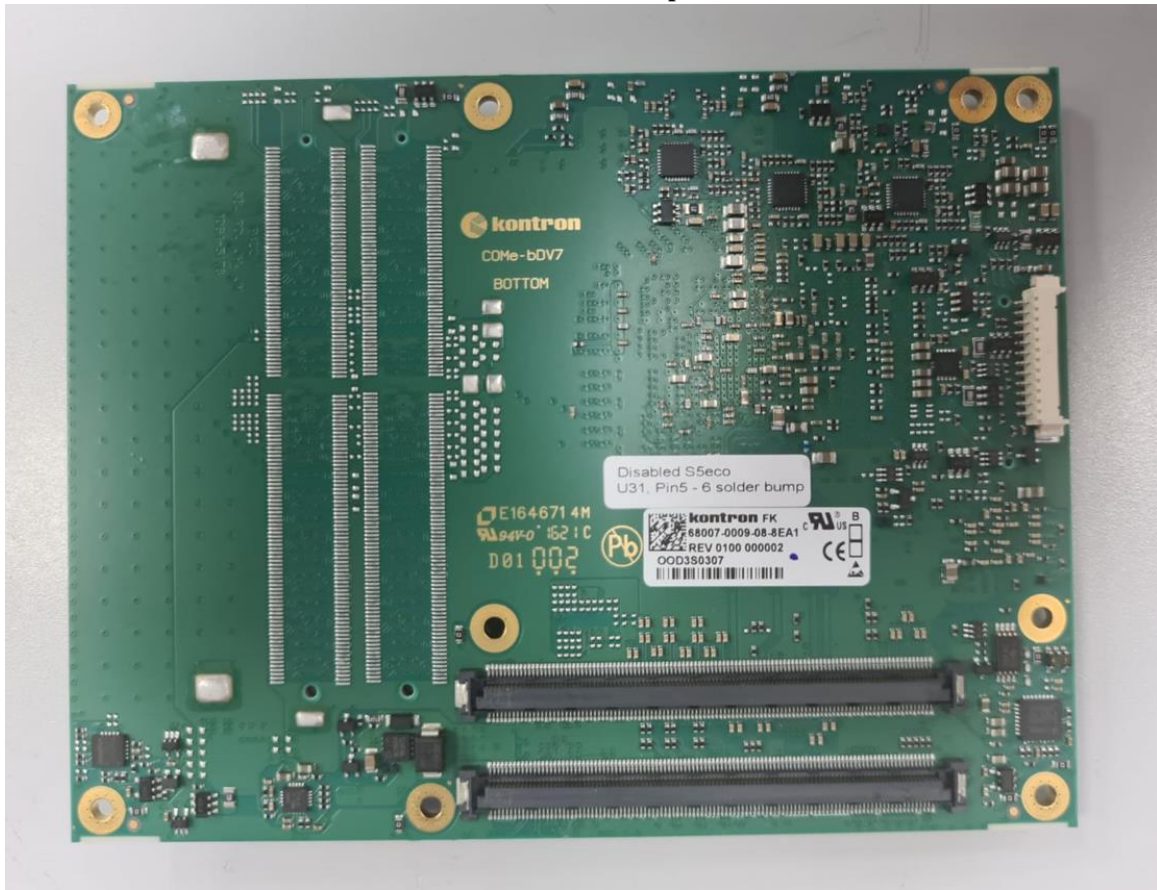
Photograph No.8 COMe board print side
