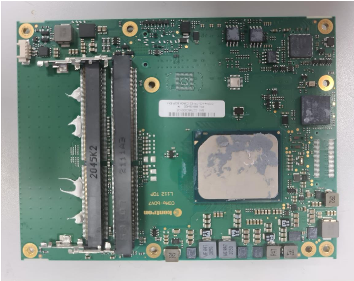
Photograph No.7 COMe board front view
