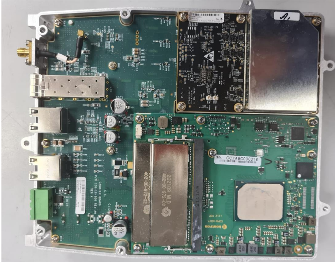
Photograph No.1 Main board front view
