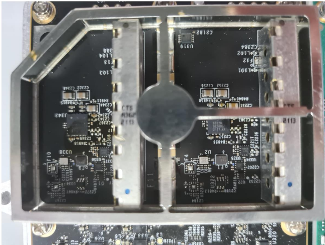
Photograph No.4 RF board
