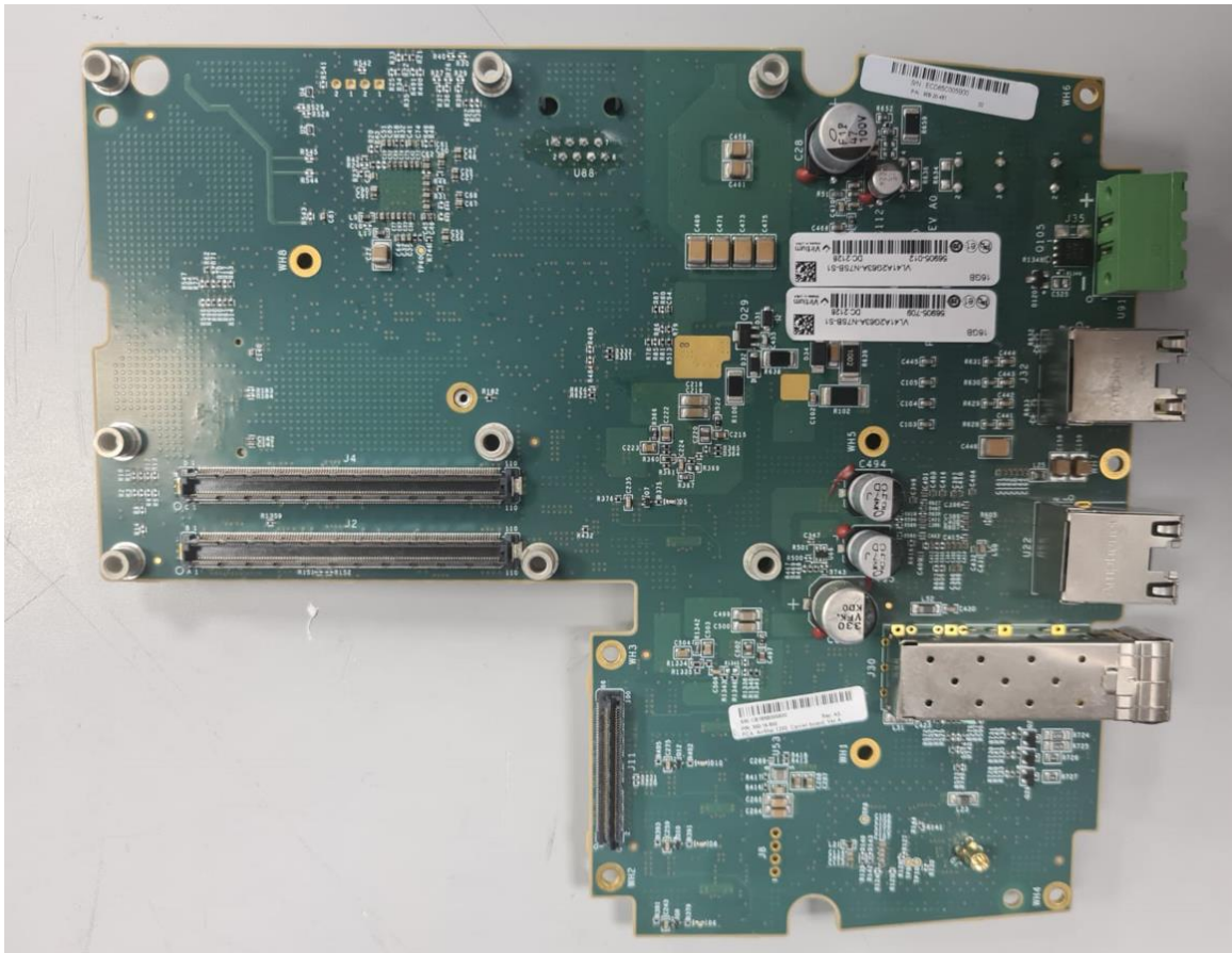
Photograph No.6 Carrier board
