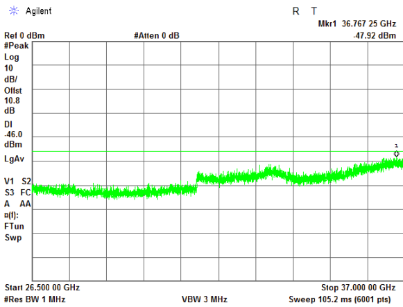
ANTENNA CHAIN: #3
