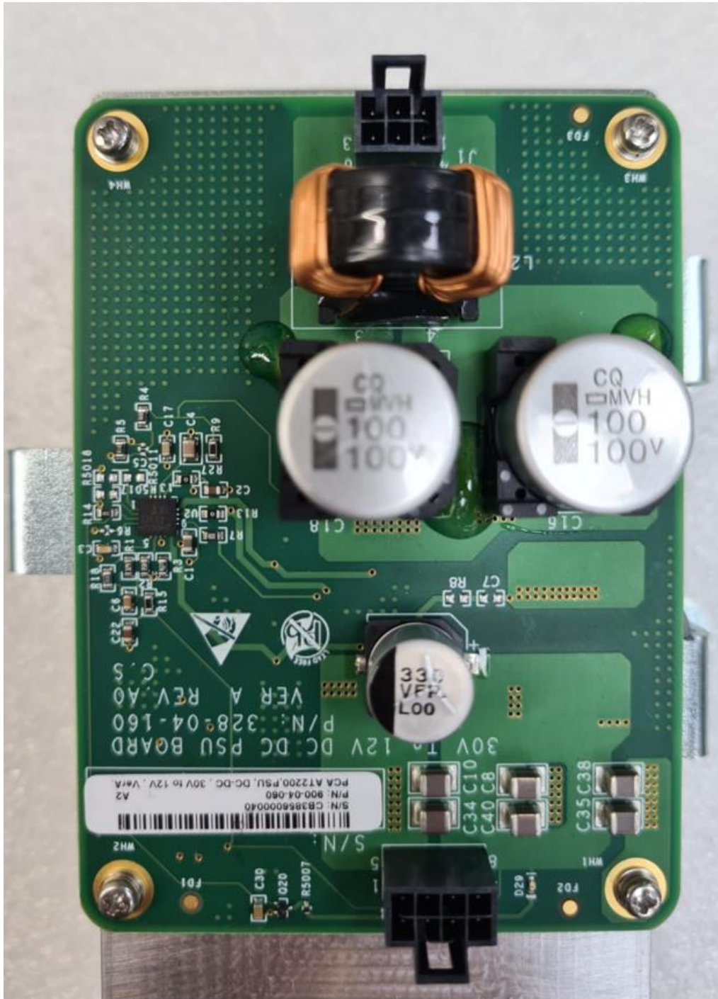
Photograph No.9 Power Supply board front view
