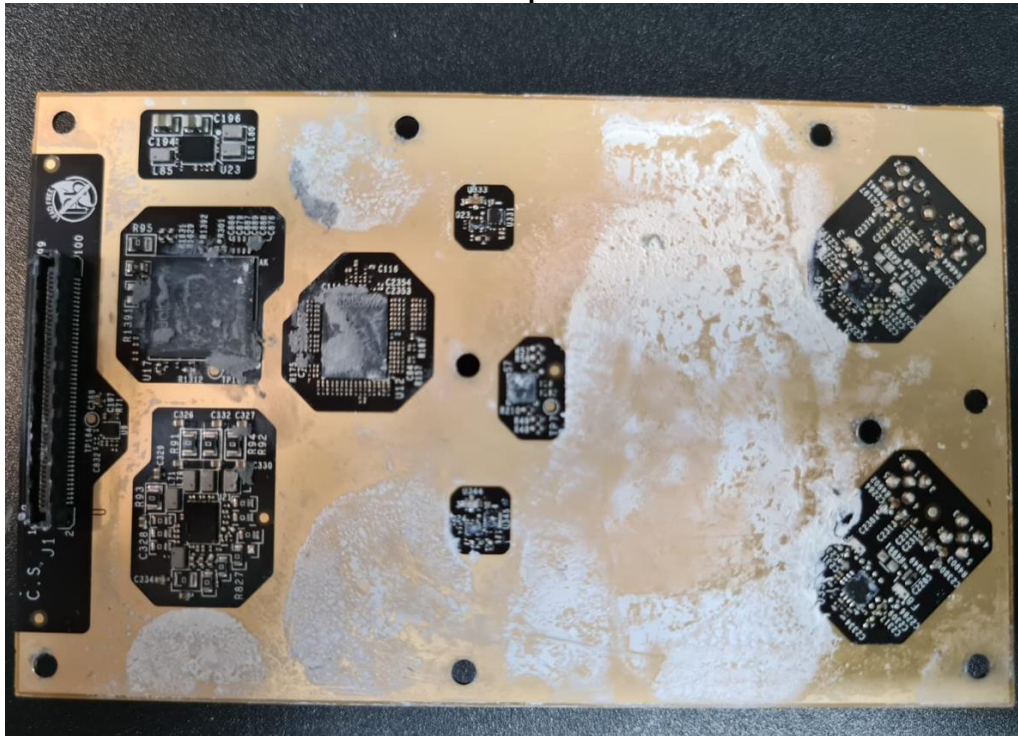
Photograph No.6 FEM board print side
