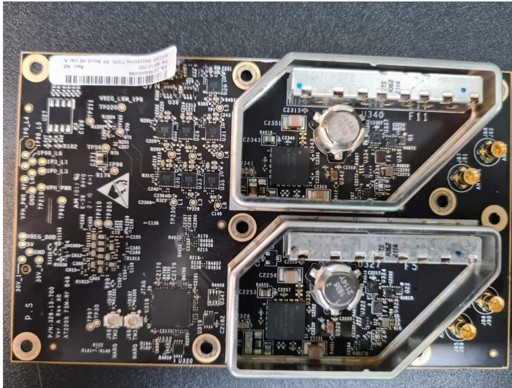
Photograph No.5 FEM board front view
