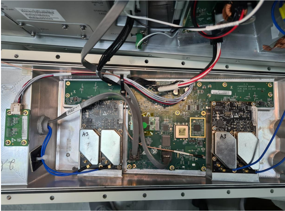
Photograph No.8 Open Unit
