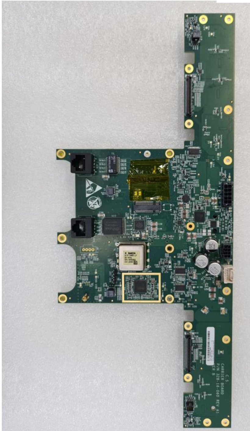
Photograph No.1 Main board front view
