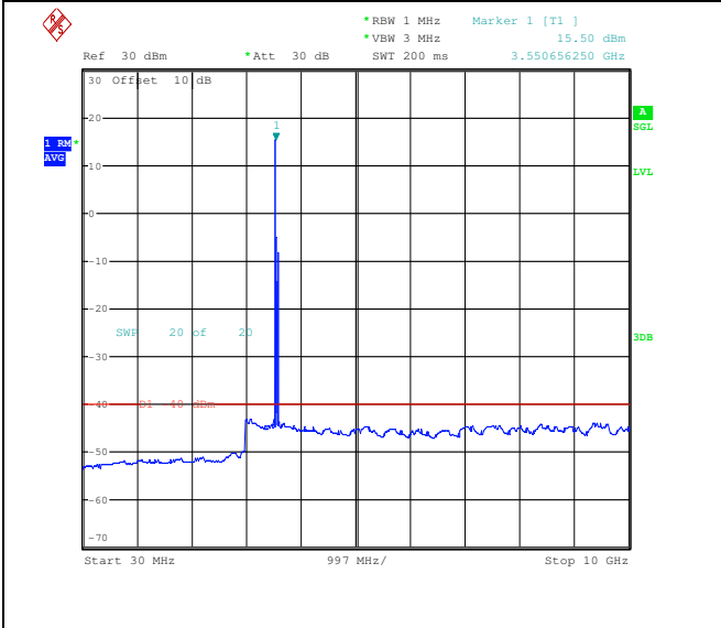
QPSK Low channel Full RB
