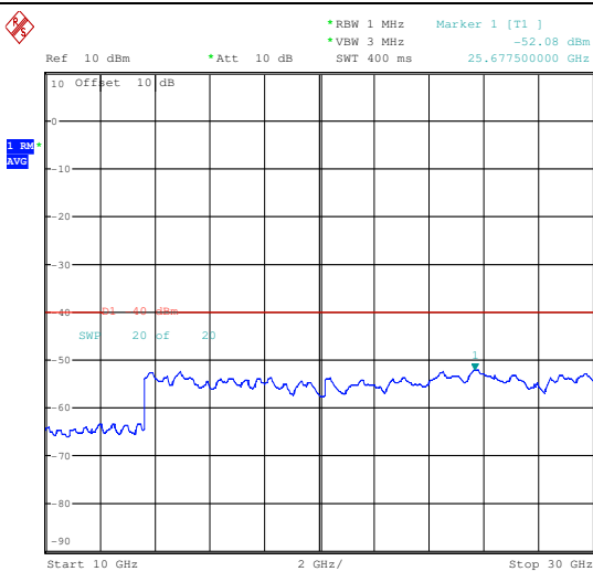
QPSK Middle channel Full RB
