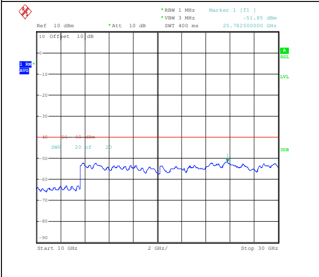
QPSK Middle channel Full RB
