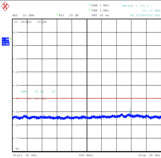
64QAM Low channel Full RB
