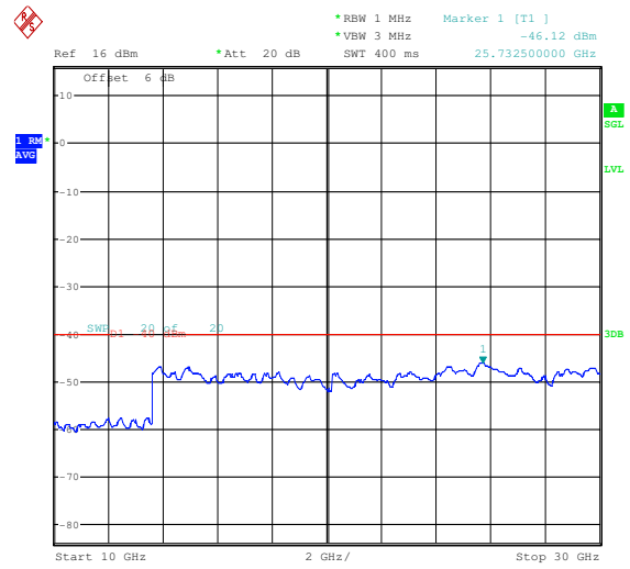
64QAM High channel 1RB0
