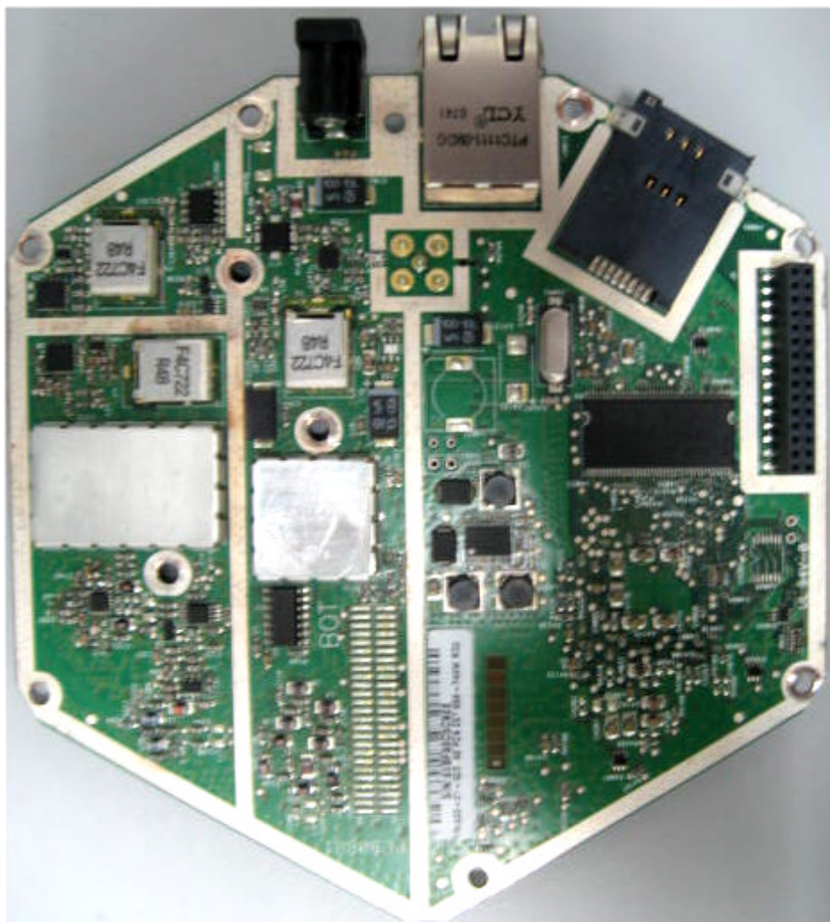
Photograph No.4 "ProST 698-746M Ext" and "Easy 698-746M" main PCB front view
