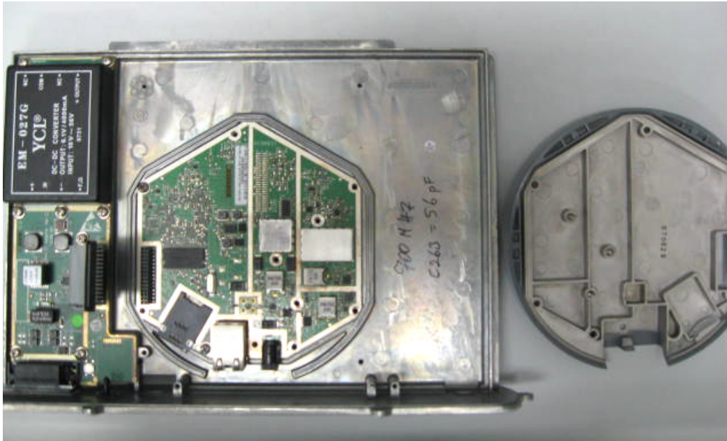
Photograph No.3 "ProST 698-746M Ext" internal view with case removed
