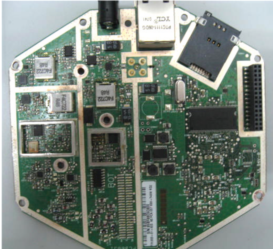
Photograph No.6 Main PCB front view without shield
