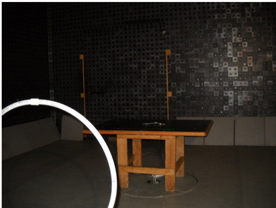
Photograph No.3 Spurious emissions measurement setup in the semi anechoic chamber below 30 MHz
