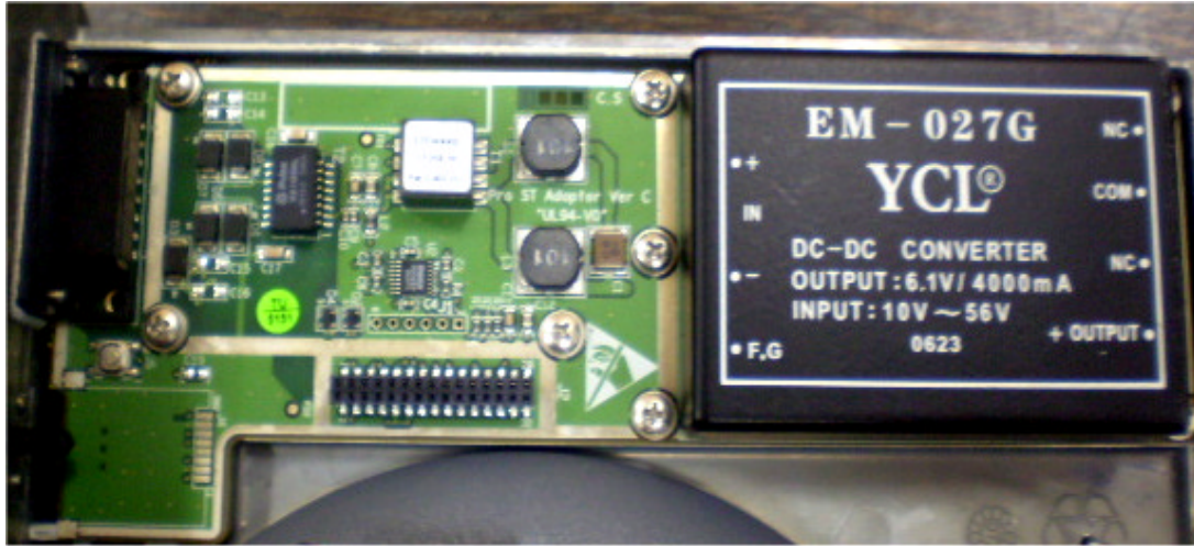
Photograph No8 ProST adapter view
