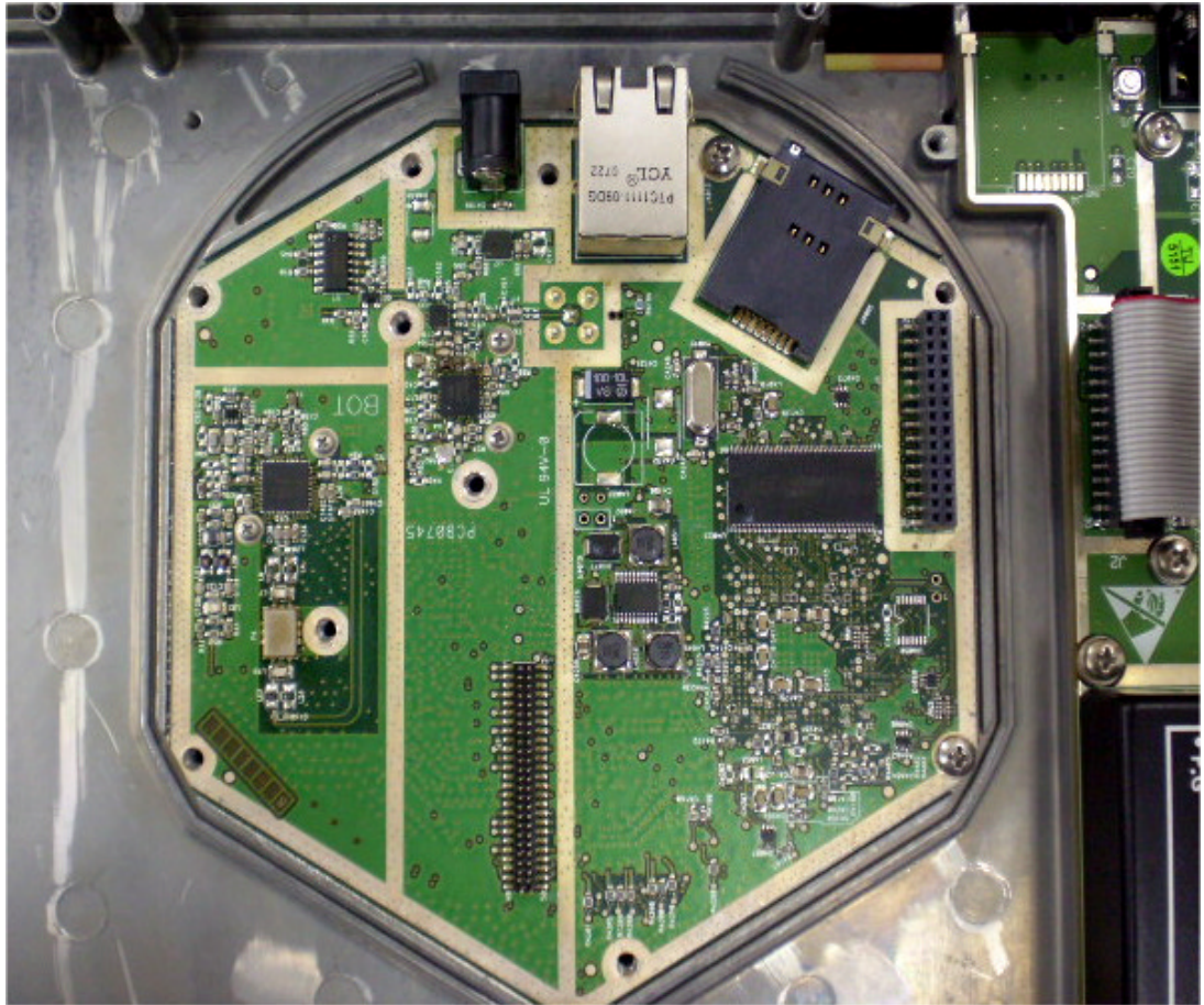
Photograph No6 ProST internal view without transmitter cover
