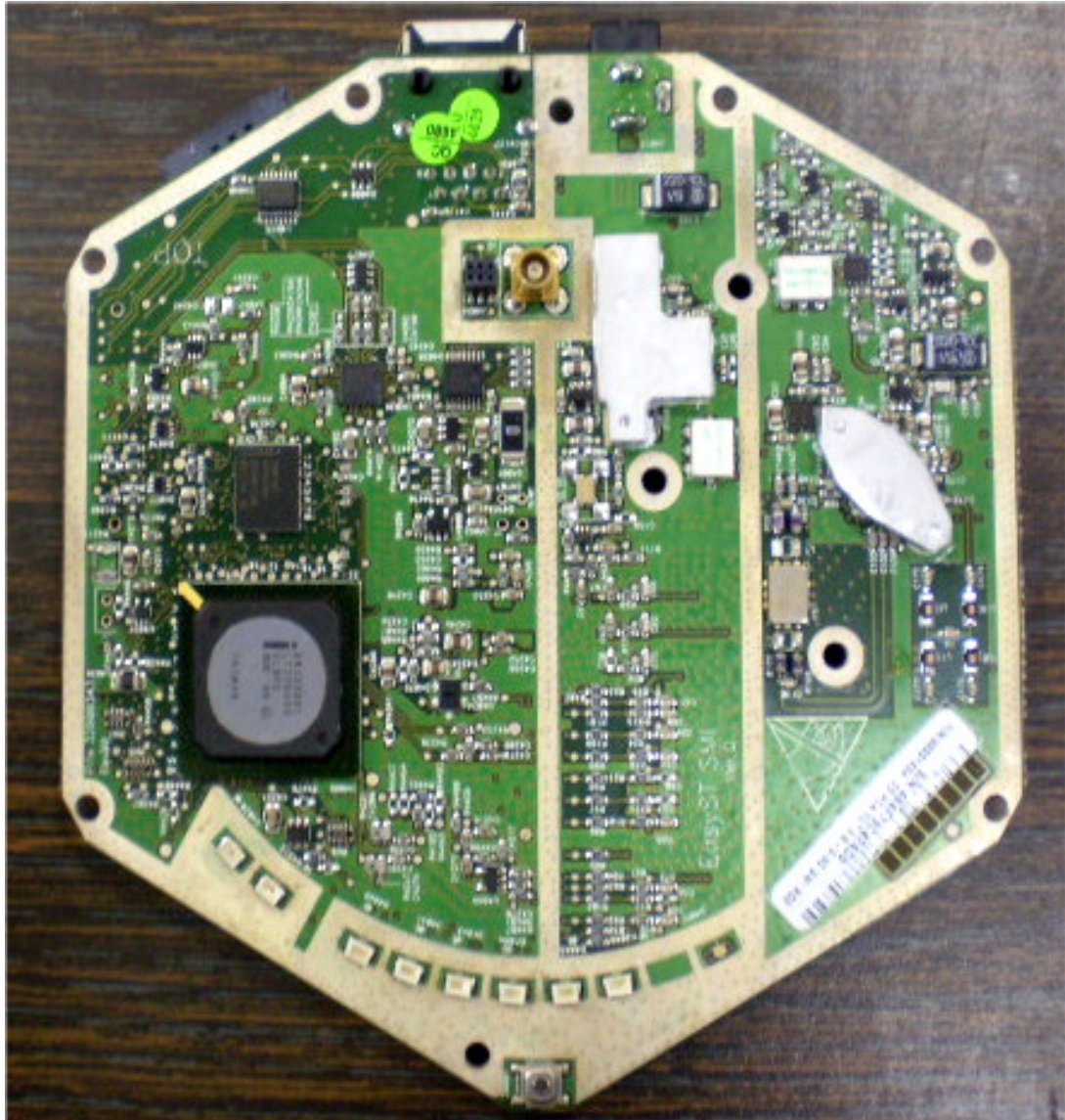
Photograph No7 ProST PCB front view
