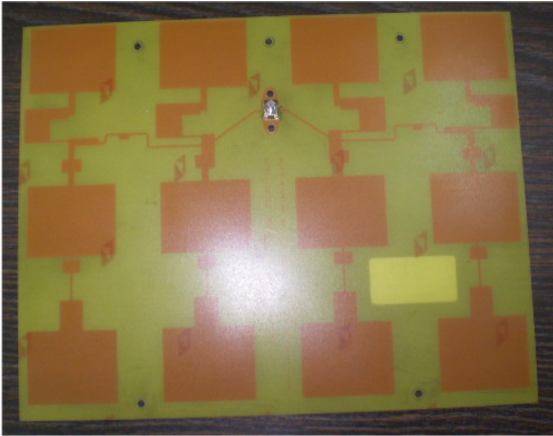
Photograph No3 ProST antennaview
