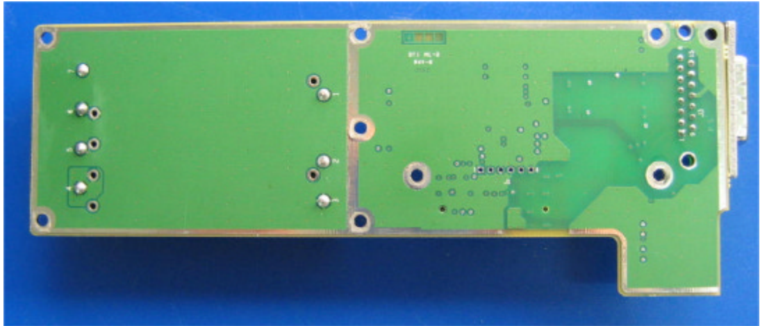
Photograph No9 ProST adapter view
