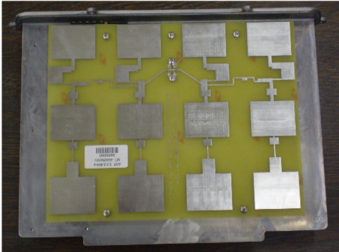
Photograph No2 ProST internal view (cover with antenna)
