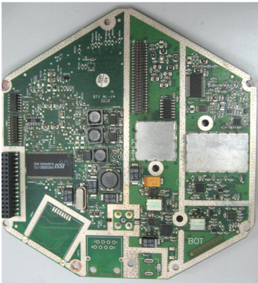
Photograph No.3 "ProST 3.65G TDD main PCB front view
