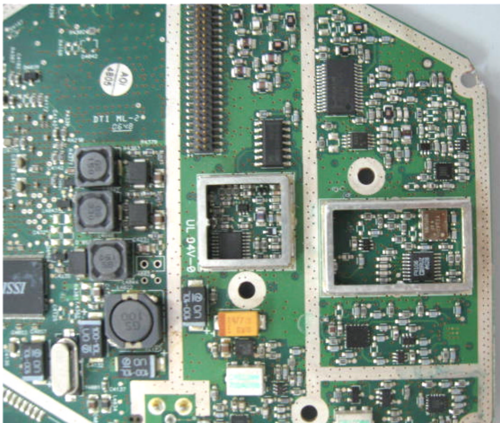
Photograph No.5 Main PCB front view without shields
