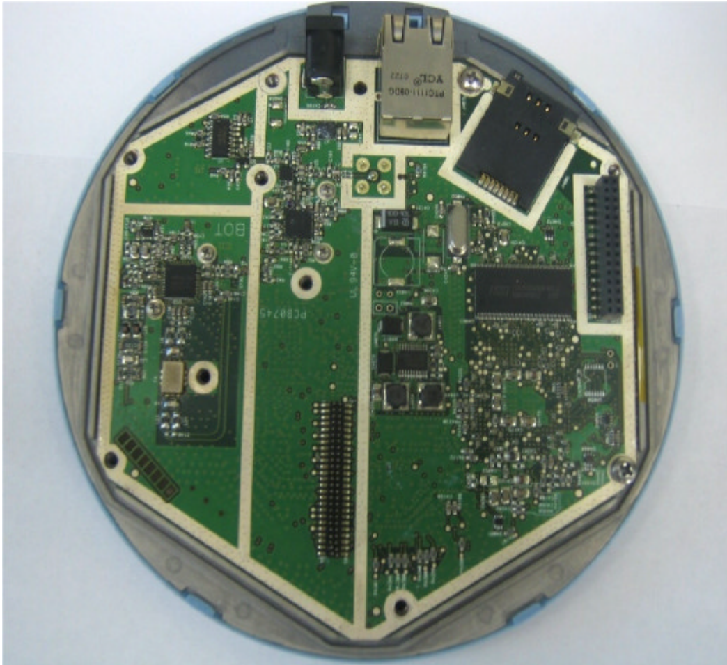
Photograph No.1 EasyST internal view
