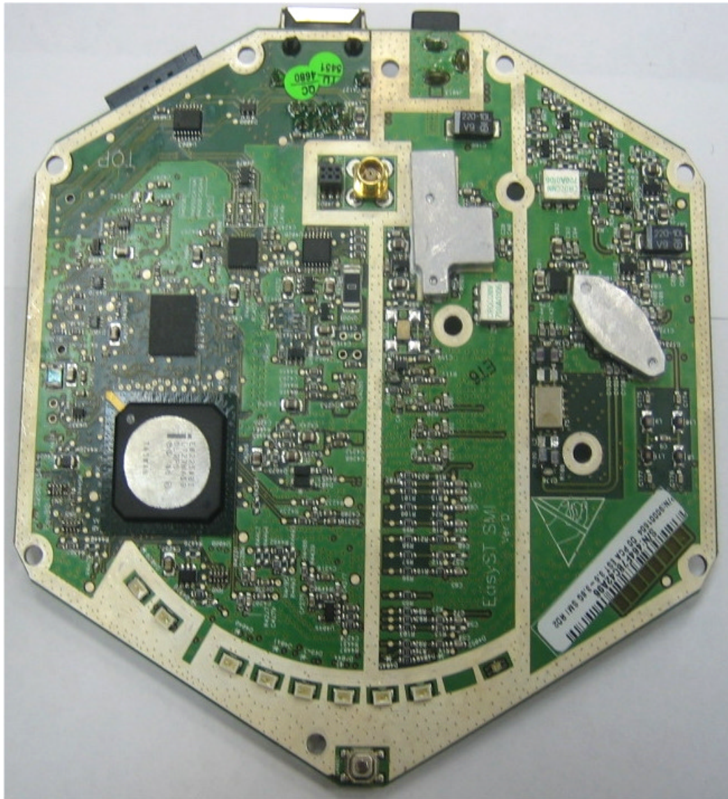
Photograph No3 EasyST PCB second side view
