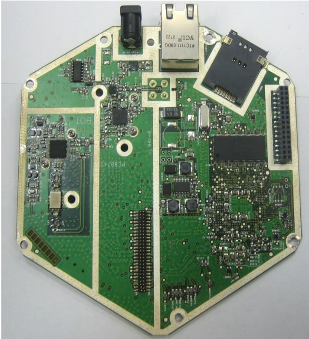
Photograph No2 EasyST PCB front view
