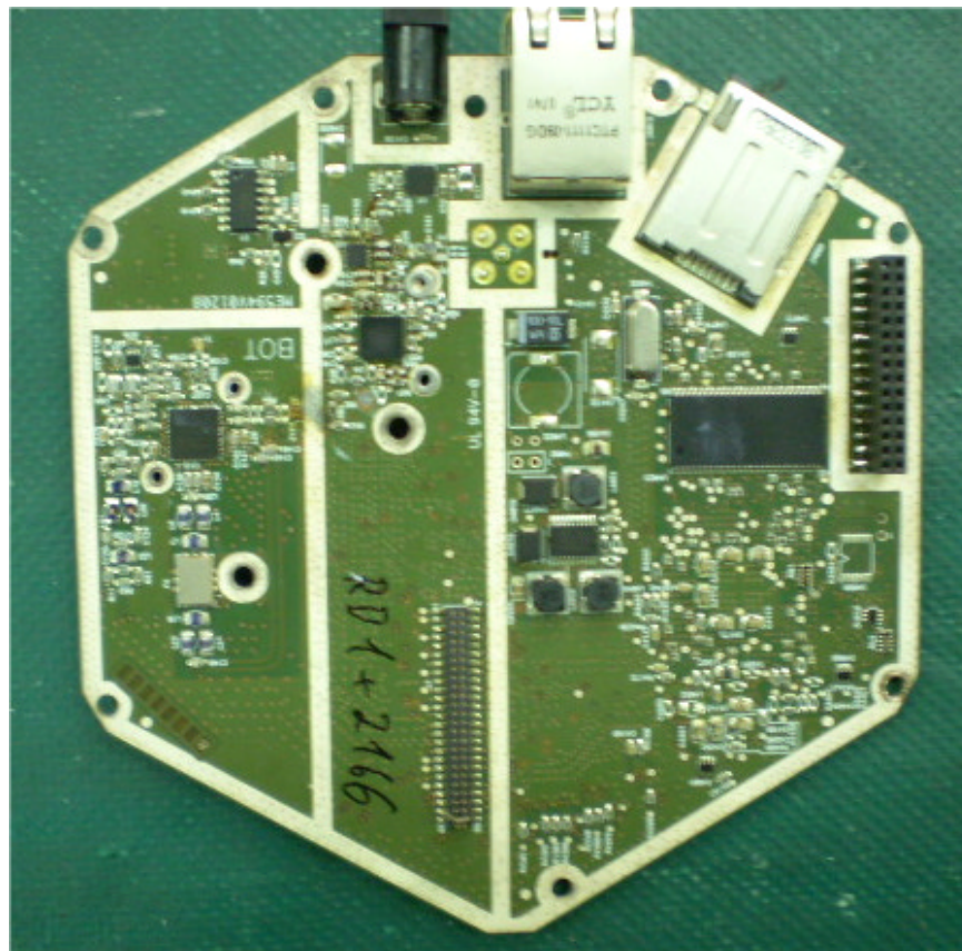
Photograph No.2 "EasyST 2.5G" PCB front view
