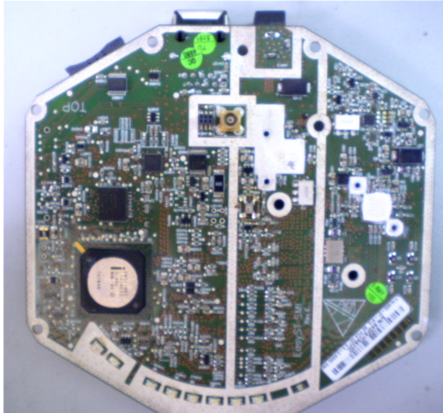
Photograph No.3 "EasyST 2.5G" PCB front view
