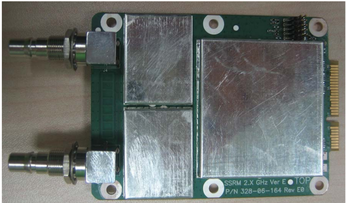
Photograph No.1 SSRM 2.5 GHz module top view
