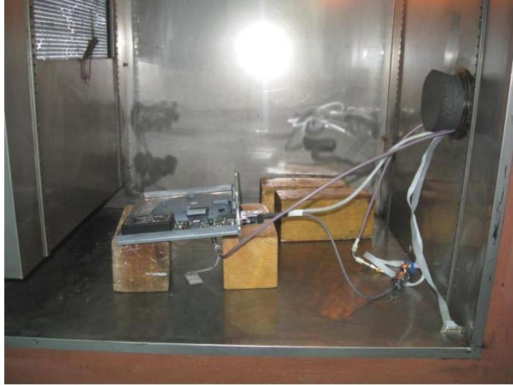
Photograph No.6 Frequency stability measurement setup
