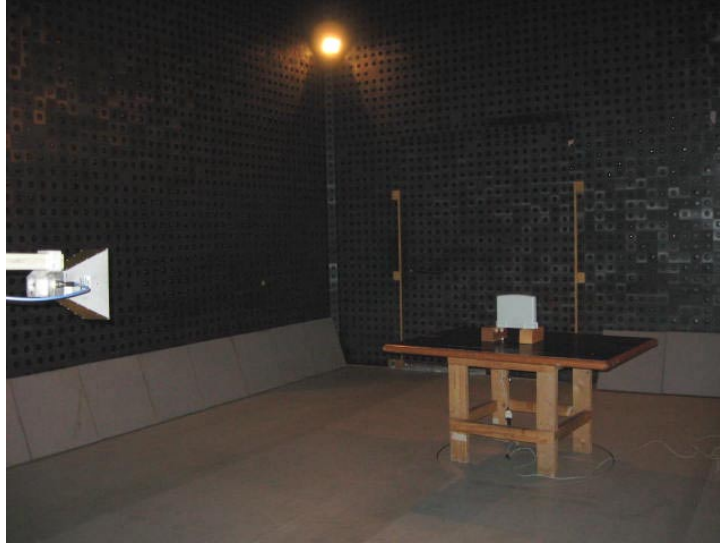
Photograph No.4 Radiated emissions measurement setup in the anechoic chamber above 1000 MHz
