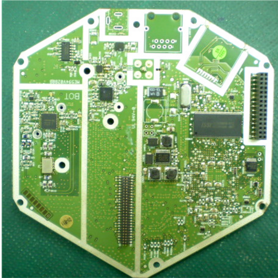
Photograph No5 “ProST 2.5G” main PCB front view
