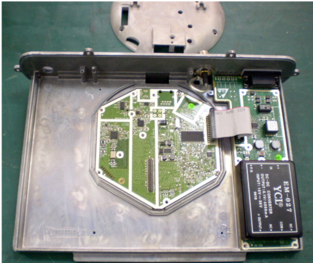
Photograph No2 "ProST 2.5G" internal view with case removed
