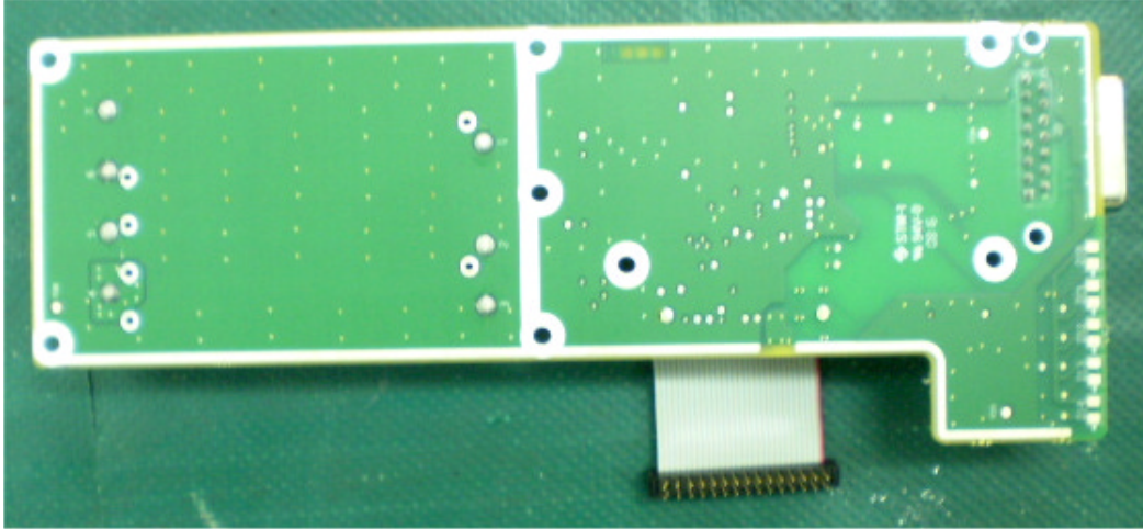
Photograph No8 “ProST 2.5G” power supply second side view
