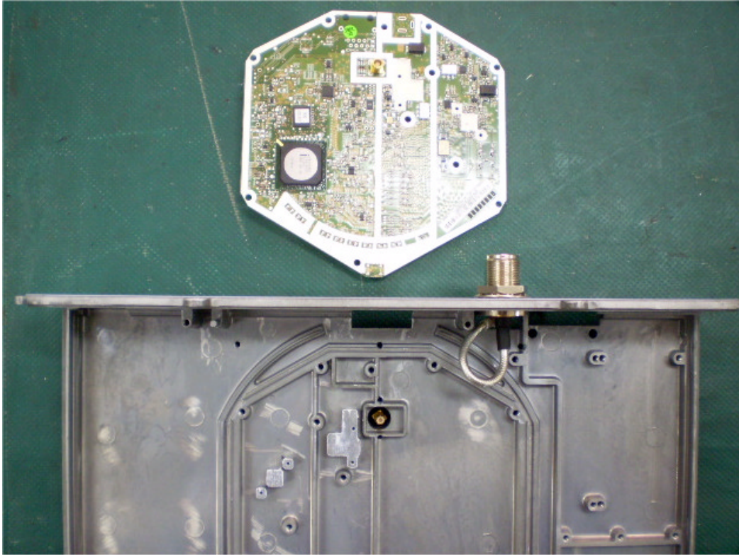
Photograph No.3 “ProST 2.5G” internal view with main PCB removed
