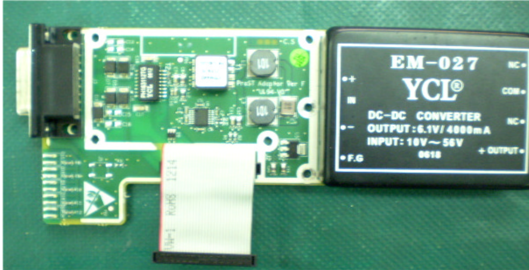
Photograph No7 "ProST 2.5G" power supply close view
