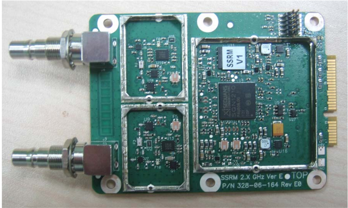
Photograph No.3 SSRM 2.3 GHz module without shielding
