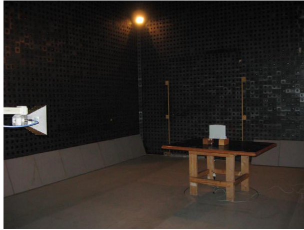
Photograph No.6 Spurious emissions measurement setup in the anechoic chamber above 1000 MHz (ProST)
