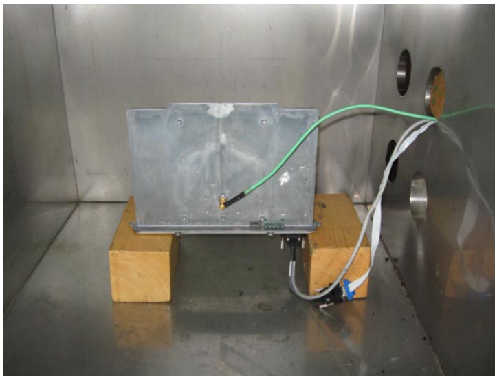
Photograph No.9 Frequency stability measurement setup
