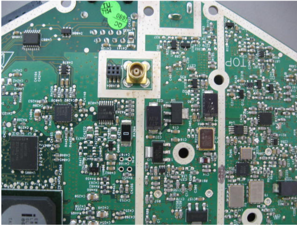
Photograph No.7 “ProST 1.4G TDD” and “Easy 1.4G TDD” main PCB second side close view
