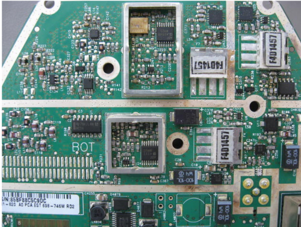
Photograph No.6 Main PCB front view without shields
