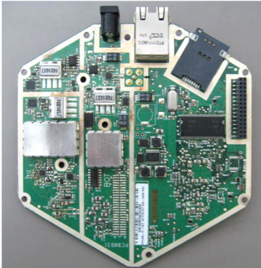
Photograph No.4 "ProST 1.4G TDD" and "Easy 1.4G TDD" main PCB front view
