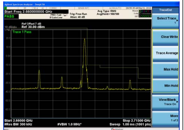
LTE Band 41 16QAM 20MHz CH-High, RB 1
