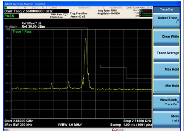
LTE Band 41 16QAM 15MHz CH-High, 100%RB
