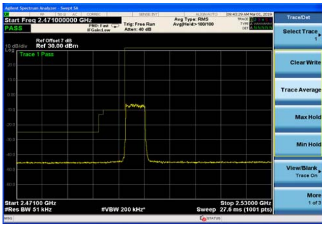
LTE Band 41 16QAM 10MHz CH-Low, 1 RB
