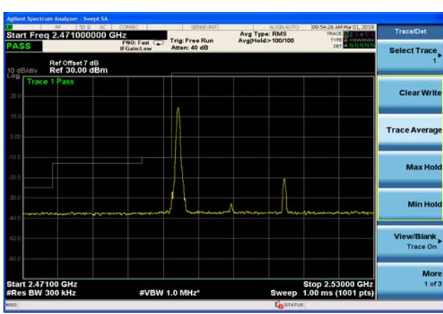
LTE Band 41 16QAM 20MHz CH-Low, RB 1
