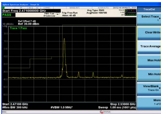
LTE Band 41 16QAM 15MHz CH-Low, 100%RB
