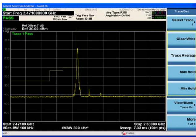
LTE Band 41 16QAM 10MHz CH-Low, 100%RB
