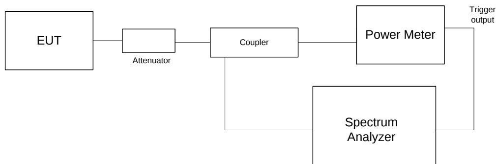
Figure 7.1.1 Peak output power test setup
