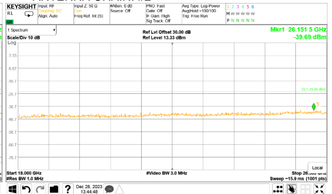
Plot 7.5.47 Spurious emission measurements in 18 – 26.5 GHz range at mid carrier frequency
