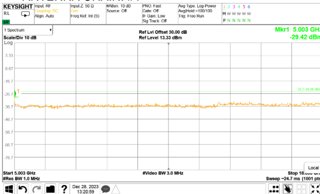
Plot 7.5.45 Spurious emission measurements in 5002.5 - 18000 MHz range at high carrier frequency
