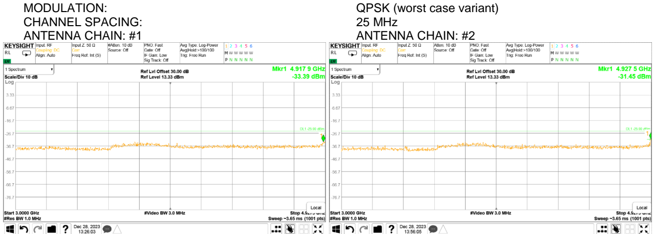
Plot 7.5.42 Spurious emission measurements in 3000 - 4927.5 MHz range at high carrier frequency
