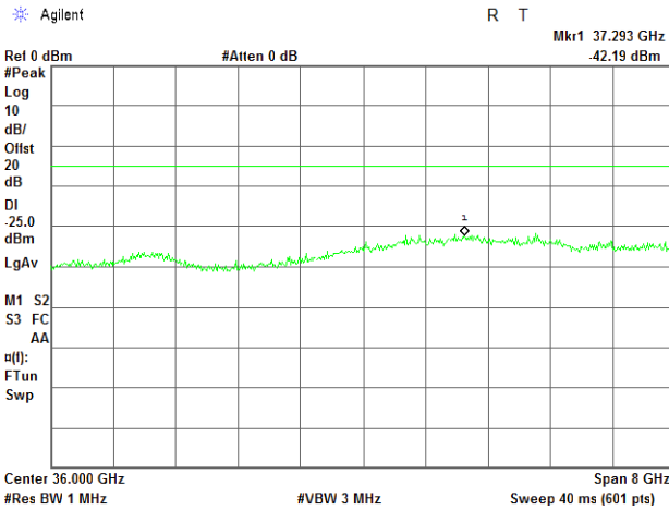
Plot 7.5.53 Spurious emission measurements in 32 - 40 GHz range at mid carrier frequency
