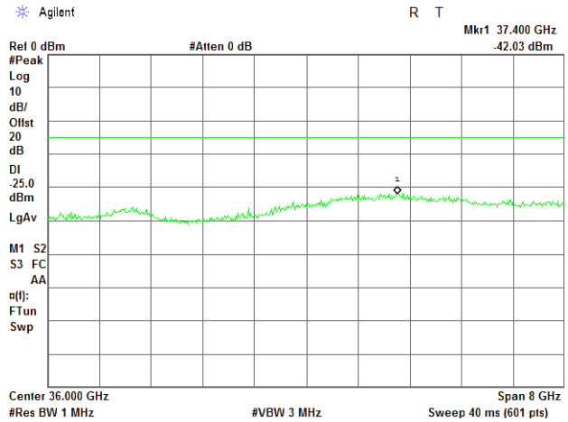
Plot 7.5.53 Spurious emission measurements in 32 - 40 GHz range at mid carrier frequency
