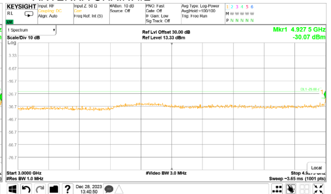
Plot 7.5.41 Spurious emission measurements in 3000 - 4927.5 MHz range at mid carrier frequency
