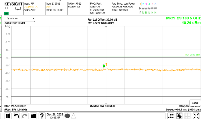
Plot 7.5.51 Spurious emission measurements in 26.5 - 32 GHz range at high carrier frequency
