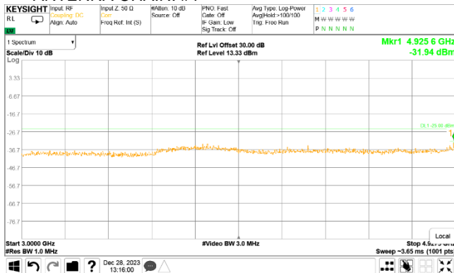
Plot 7.5.41 Spurious emission measurements in 3000 - 4927.5 MHz range at mid carrier frequency
