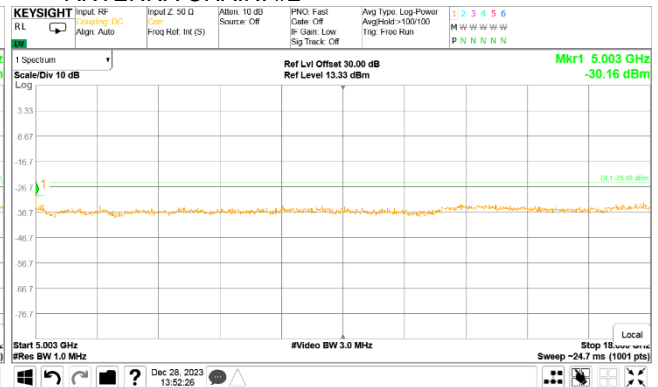
Plot 7.5.45 Spurious emission measurements in 5002.5 - 18000 MHz range at high carrier frequency
