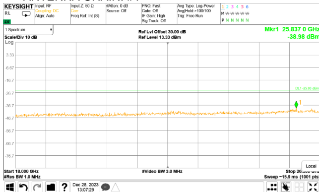
Plot 7.5.47 Spurious emission measurements in 18 – 26.5 GHz range at mid carrier frequency
